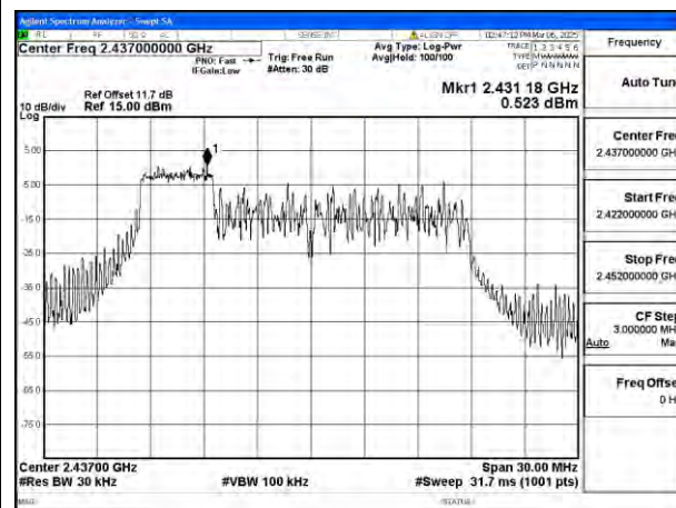
Mode:802.11ax HE20 Tone:52T Frequency:2437MHz Ant:Chain0
