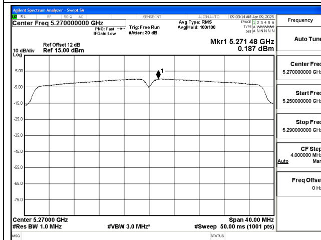
Mode:802.11ac VHT40 Frequency:5270MHz Ant:Chain1
