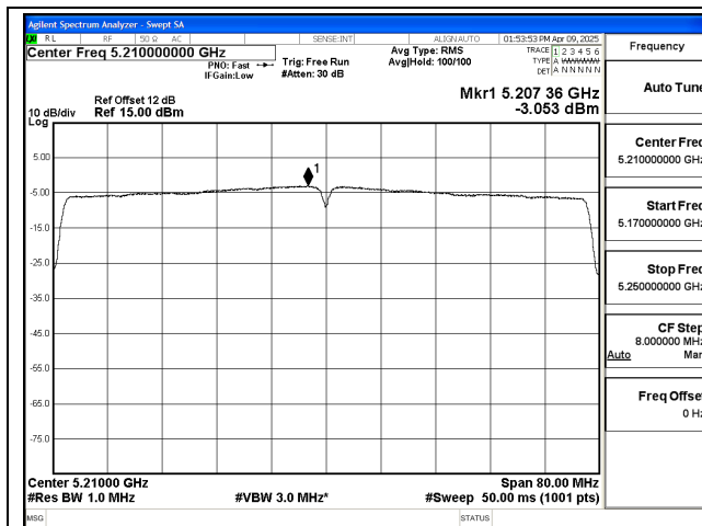
Mode:802.11ac VHT80 Frequency:5210MHz Ant:Chain0
