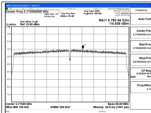
Mode:802.11ac VHT80 Frequency:5775MHz Ant:Chain0
