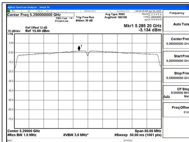
Mode:802.11ac VHT80 Frequency:5290MHz Ant:Chain0
