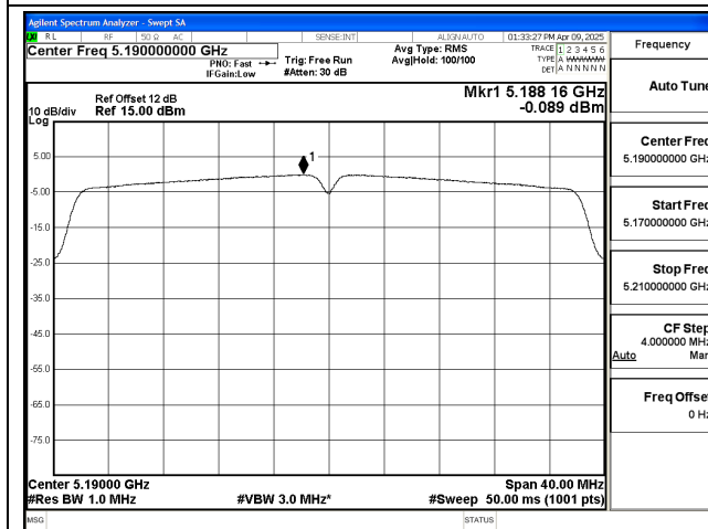
Mode:802.11ac VHT40 Frequency:5190MHz Ant:Chain1
