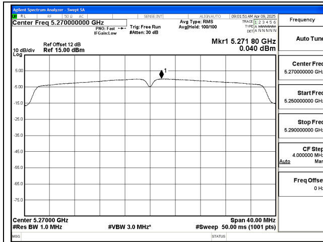
Mode:802.11ac VHT40 Frequency:5270MHz Ant:Chain0
