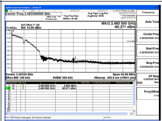
Mode:802.11b Frequency:2462MHz Ant:Chain1
