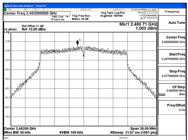
Mode:802.11n HT20 Frequency:2462MHz Ant:Chain1
