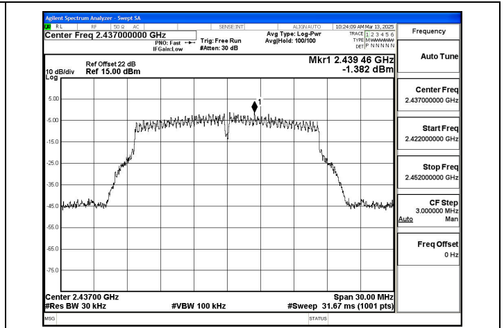
Mode:802.11g Frequency:2437MHz Ant:Chain0
