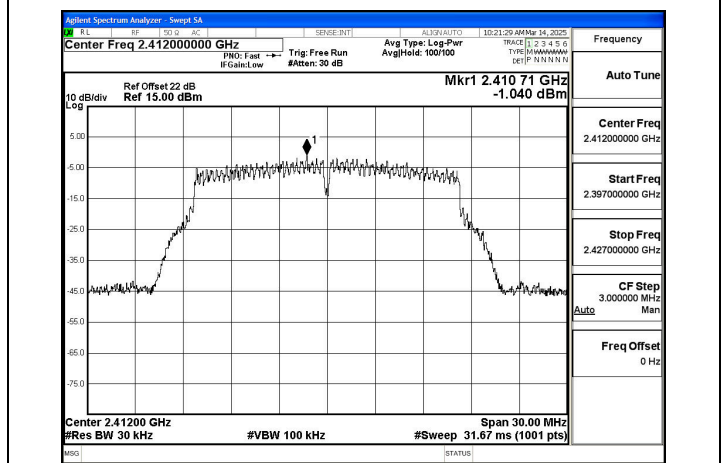
Mode:802.11g Frequency:2412MHz Ant:Chain1
