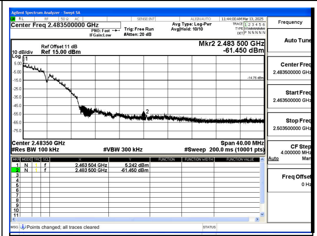
Mode:802.11b Frequency:2462MHz Ant:Chain0
