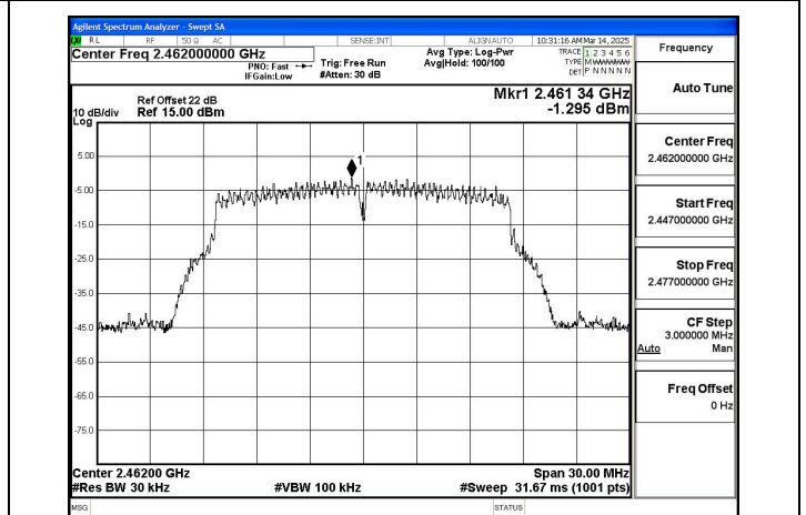
Mode:802.11g Frequency:2462MHz Ant:Chain1
