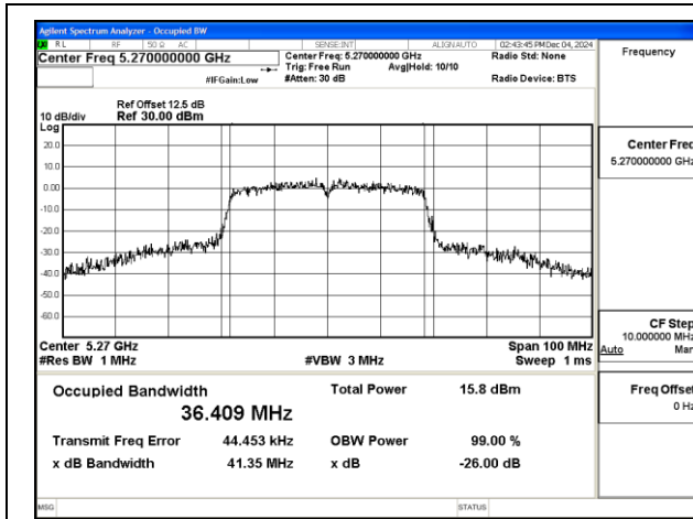
Mode:802.11n HT40 Frequency:5270MHz Ant:Chain1
