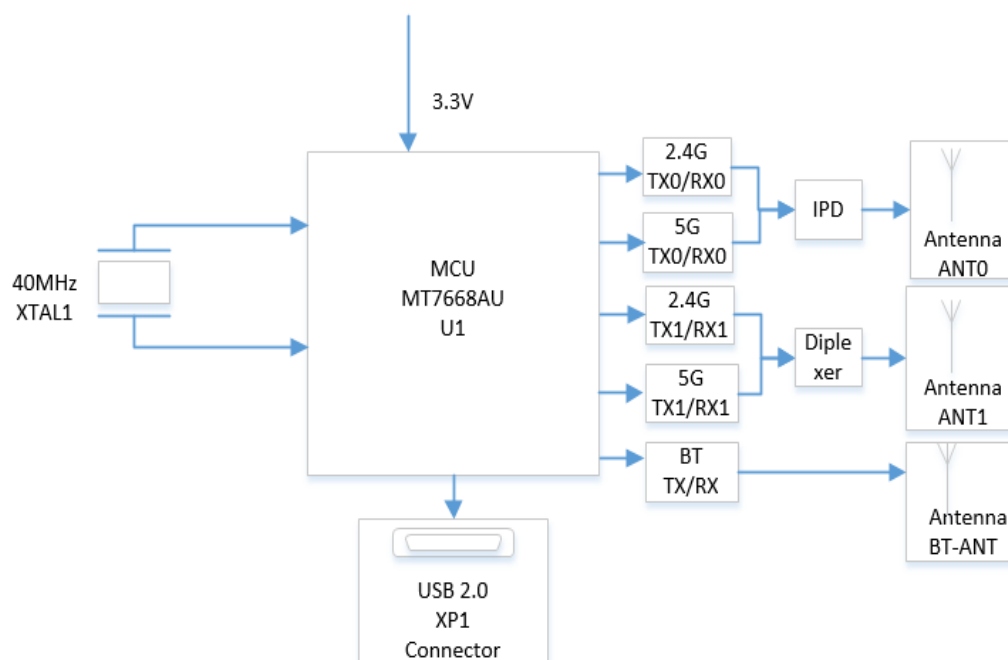
BLOCK DIAGRAM
