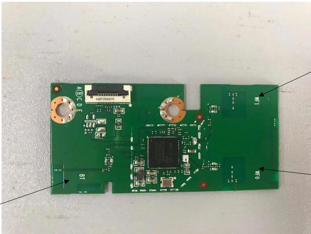
WiFi Antenna 1
