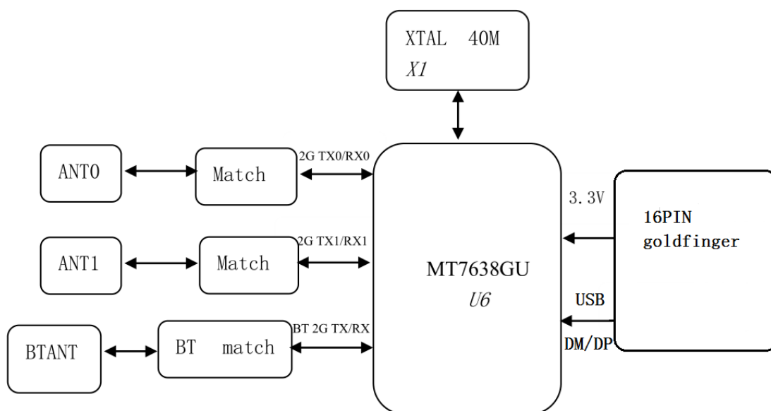
BLOCK DIAGRAM
