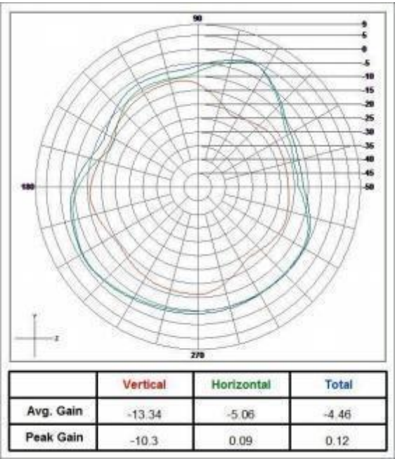
2.44 GHz 2D Plot
