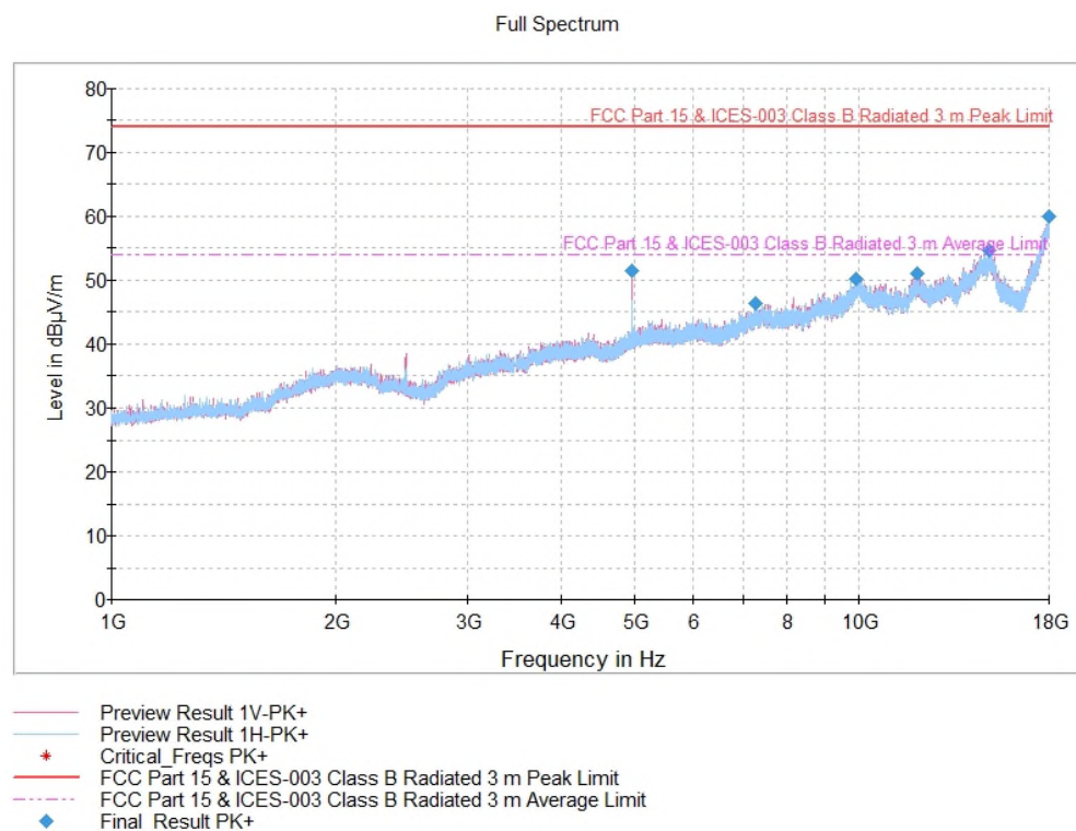
Figure 7.2.1.3-2: Emission Profile – 1 to 18GHz
