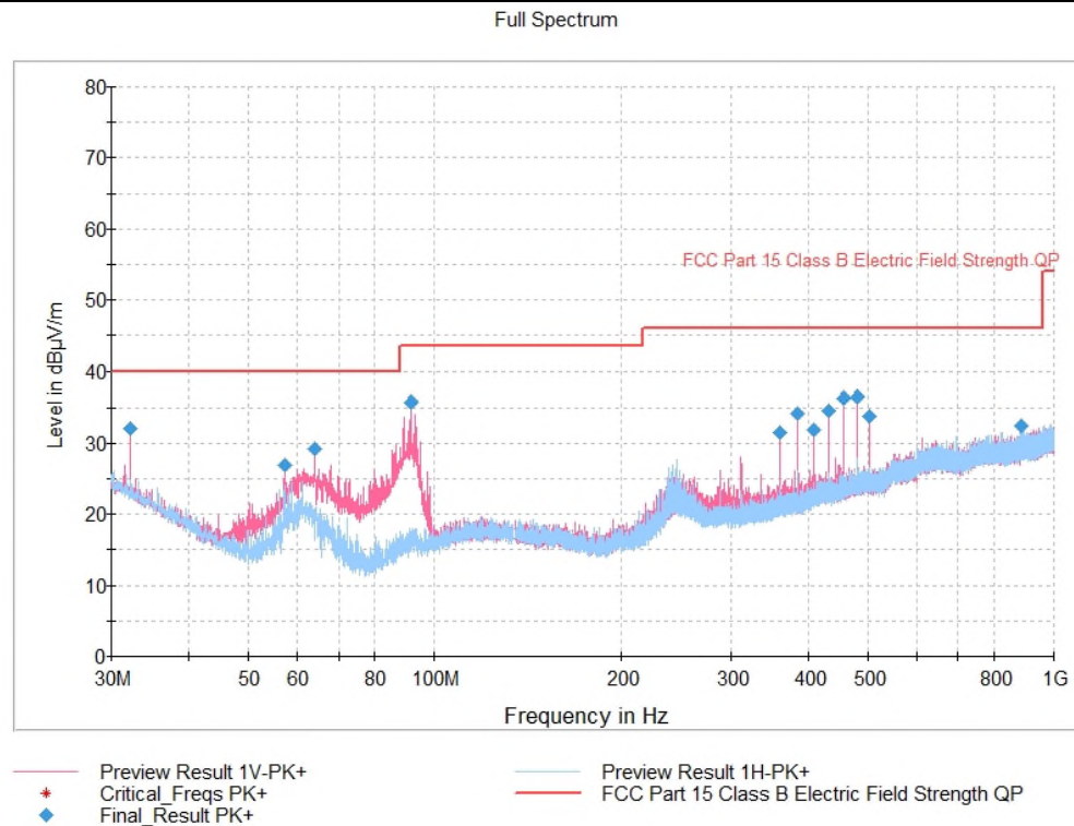
Figure 7.2.1.3-1: Emission Profile – Below 1GHz
