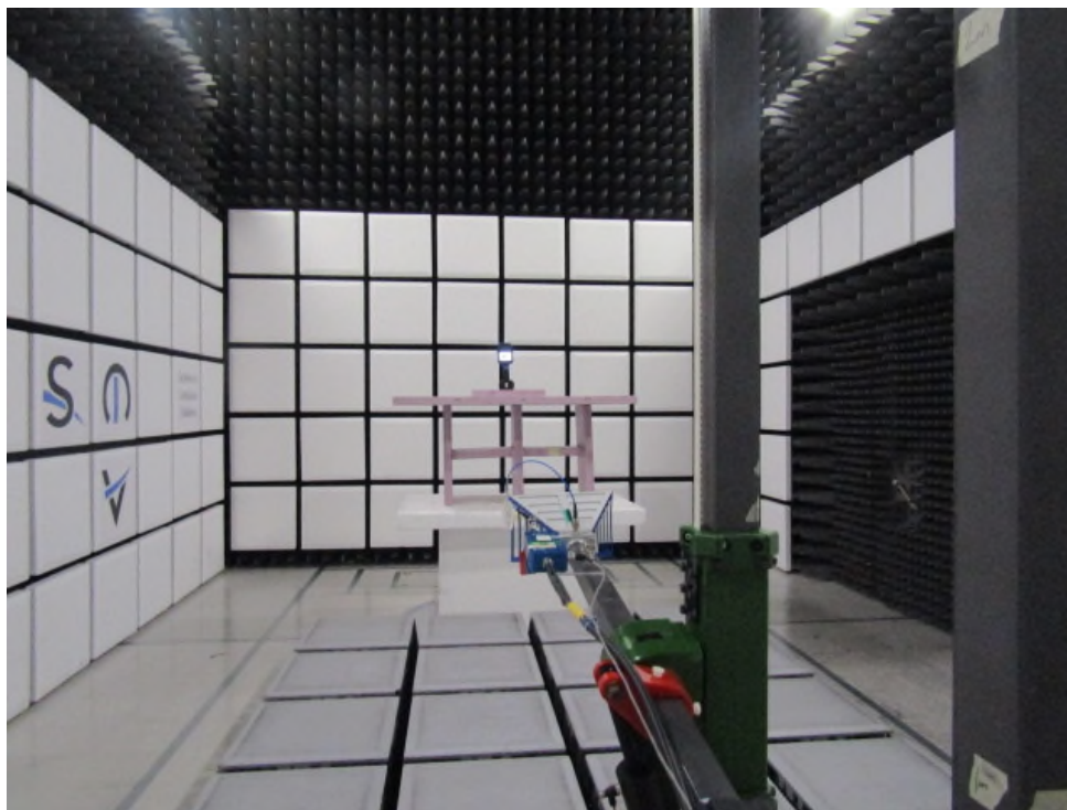
Figure 3: Radiated Emissions – Back – Above 1GHz
