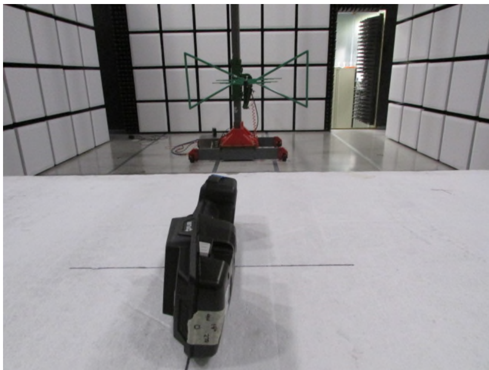
Figure 6: Radiated Emissions – YPOS
