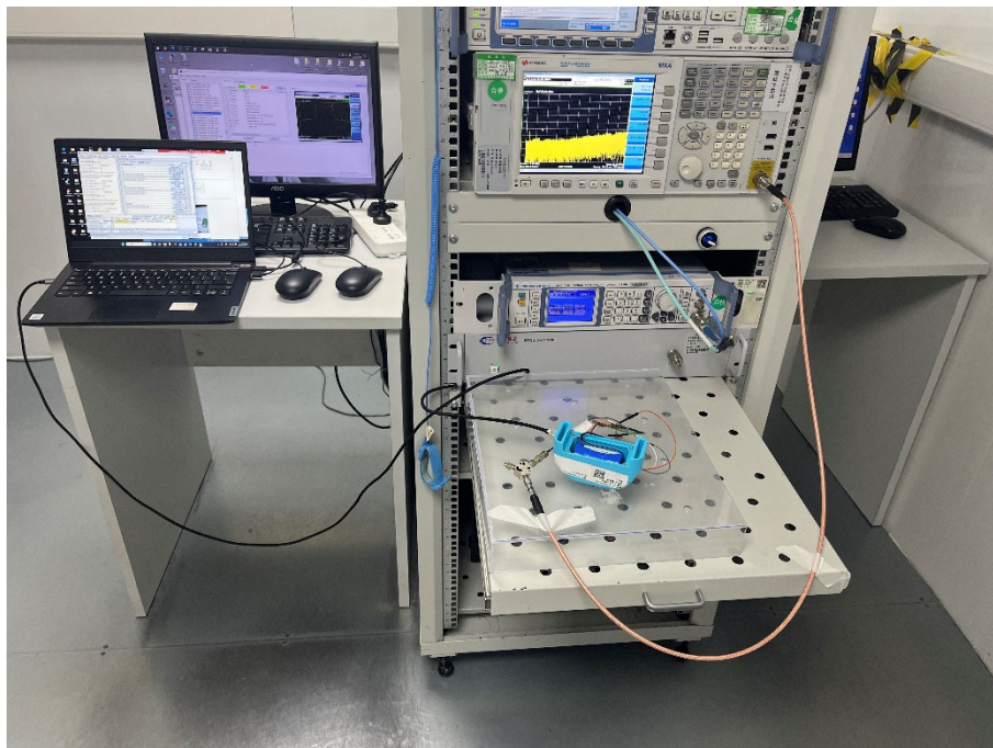
Conducted Test-BLE&LoRa
