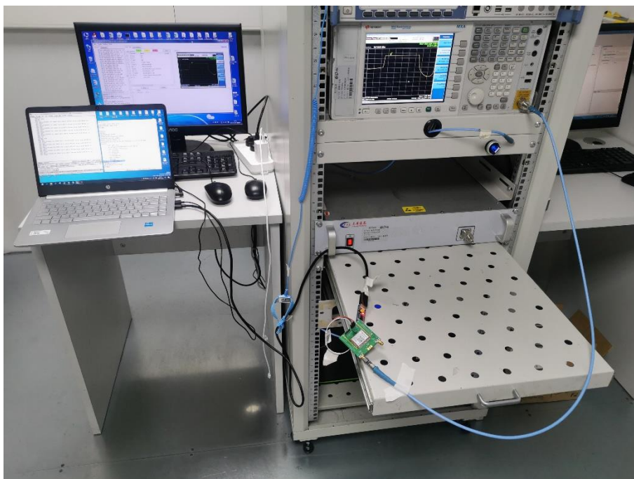
Conducted Test-LoRa 927.5 MHz
