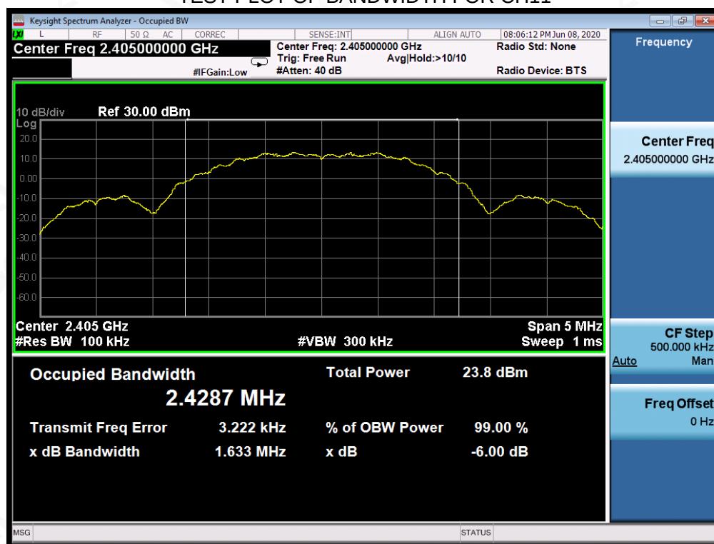
TEST PLOT OF BANDWIDTH FOR CH11
