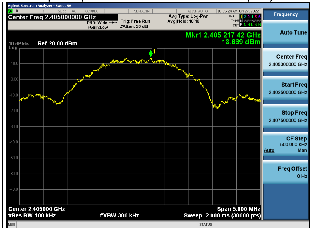
Test_Graph_2.4G_ANT1_2405_Reference Level
