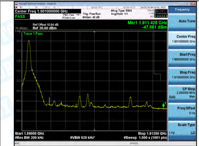
Band2_Band2_20MHz_16QAM_19100_1RB#0
