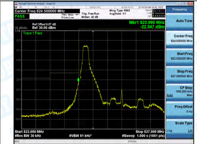
Band5_Band5_3MHz_16QAM_20415_1RB#0
