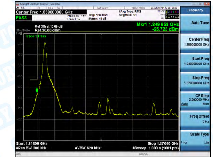
Band2_Band2_20MHz_16QAM_18700_1RB#0
