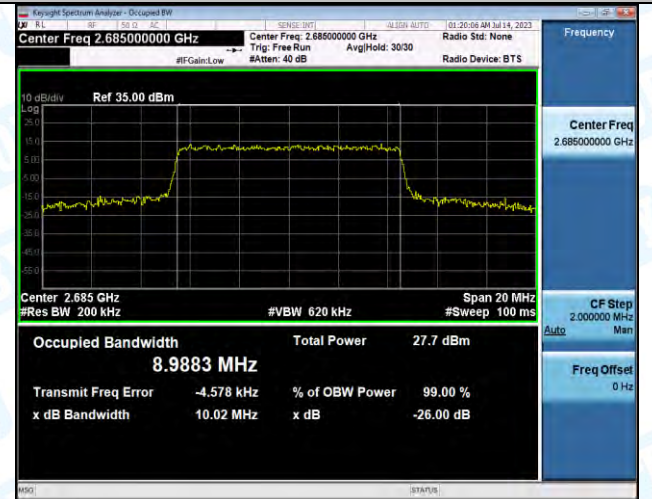
Band41-10MHz-16QAM-41540-50RB#0-PASS
