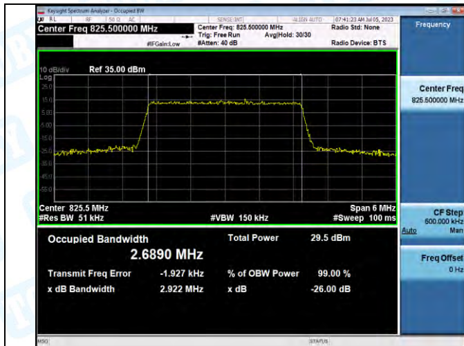
Band5-3MHz-QPSK-20415-15RB#0-PASS
