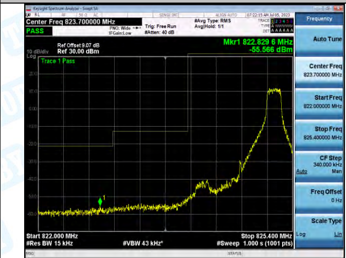
Band5_Band5_1.4MHz_16QAM_20407_1RB#5
