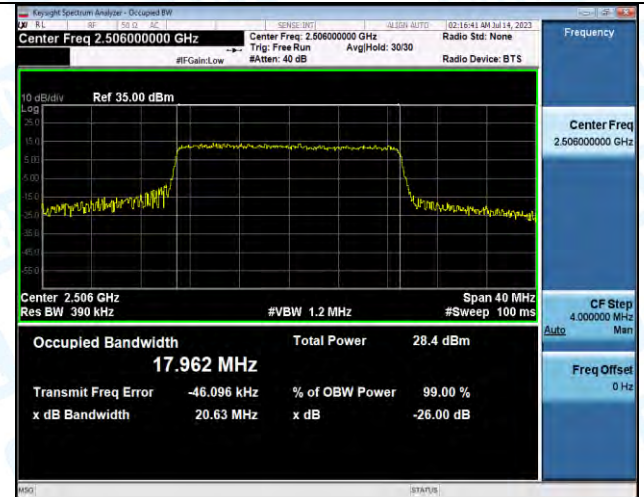
Band41-20MHz-16QAM-39750-100RB#0-PASS
