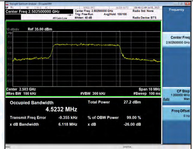
Band7-5MHz-16QAM-20775-25RB#0-PASS
