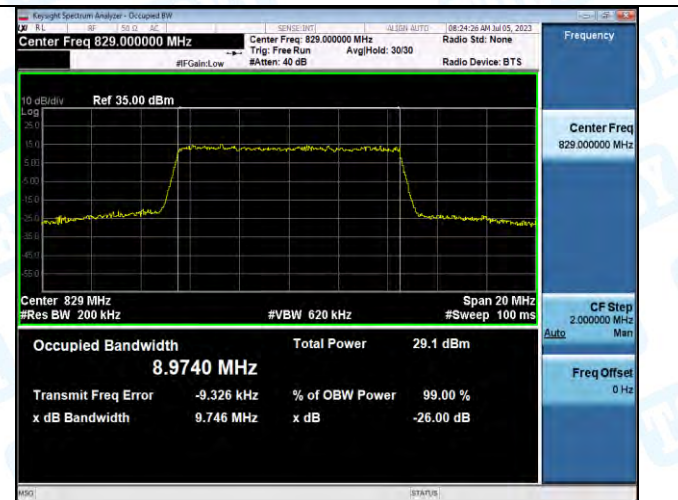
Band5-10MHz-16QAM-20450-50RB#0-PASS
