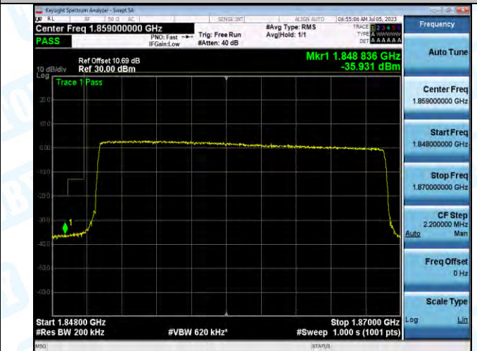
Band2_Band2_20MHz_16QAM_18700_100RB#0
