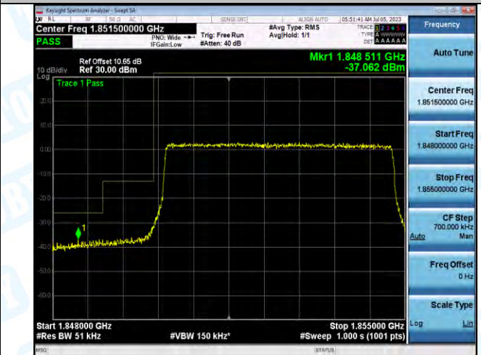
Band2_Band2_5MHz_16QAM_18625_25RB#0
