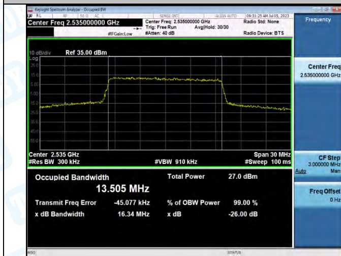
Band7-15MHz-QPSK-21100-75RB#0-PASS
