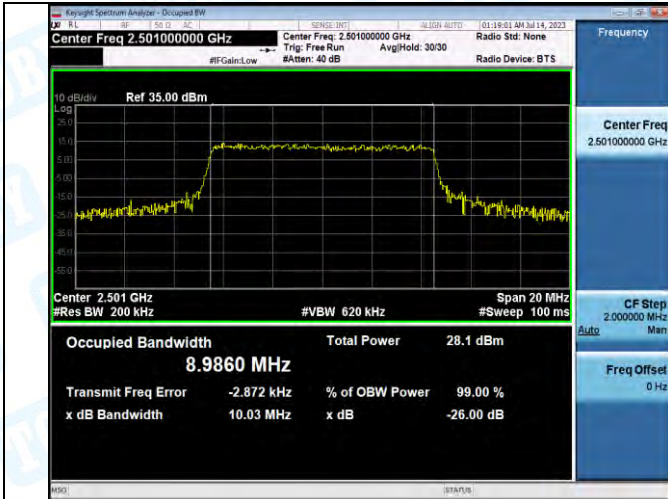
Band41-10MHz-QPSK-39700-50RB#0-PASS
