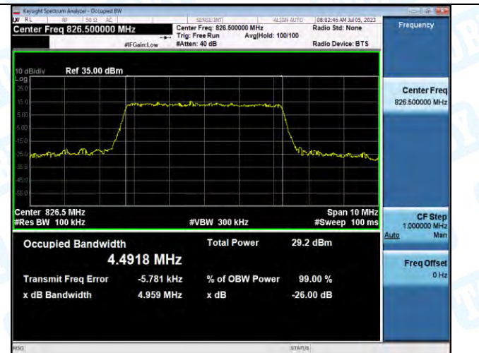
Band5-5MHz-16QAM-20425-25RB#0-PASS
