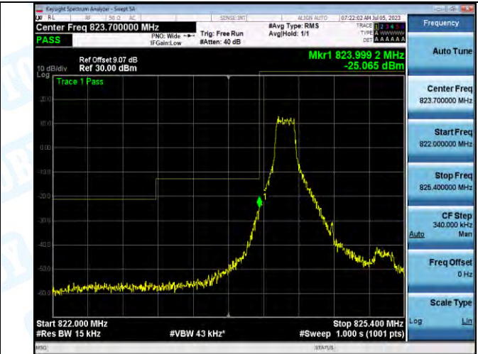
Band5_Band5_1.4MHz_16QAM_20407_1RB#0
