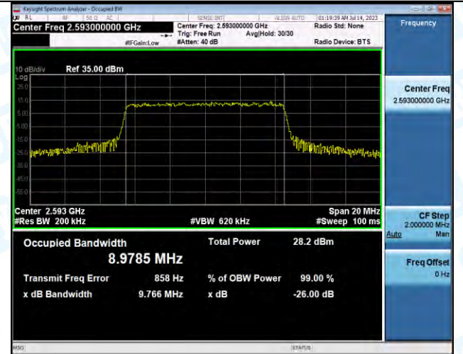
Band41-10MHz-16QAM-40620-50RB#0-PASS
