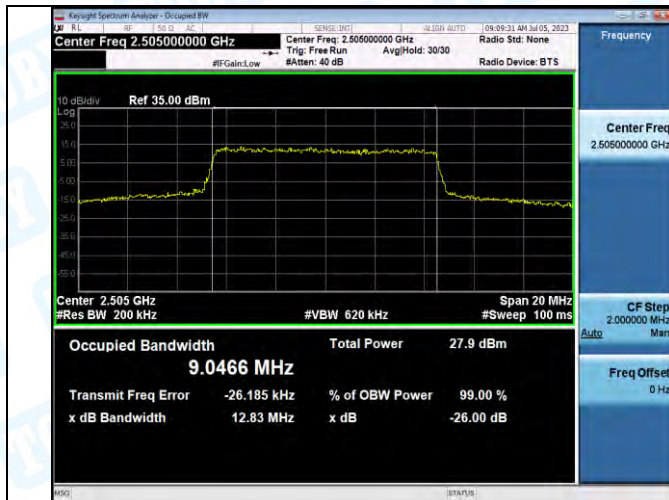
Band7-10MHz-QPSK-20800-50RB#0-PASS
