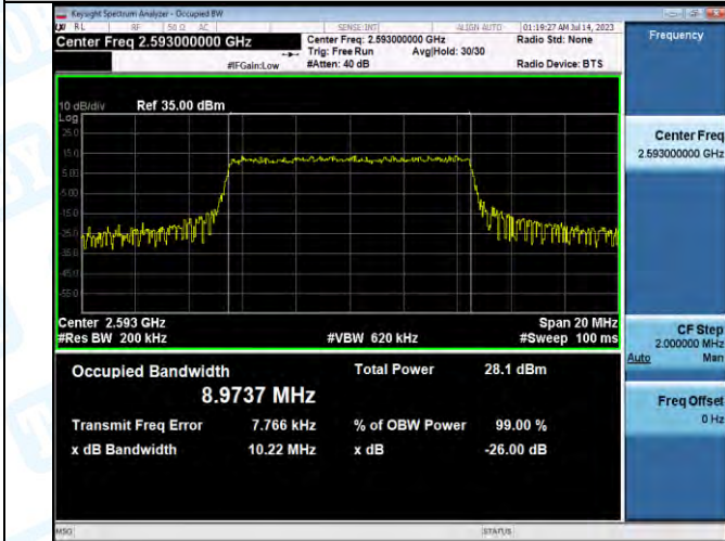
Band41-10MHz-QPSK-40620-50RB#0-PASS
