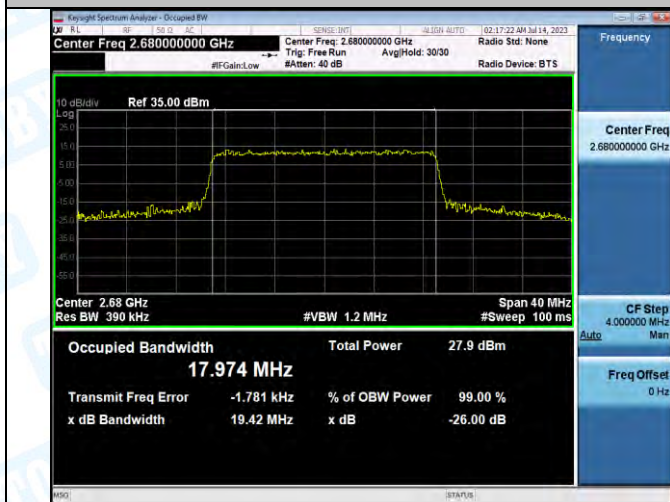
Band41-20MHz-QPSK-41490-100RB#0-PASS
