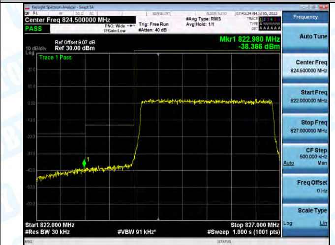
Band5_Band5_3MHz_16QAM_20415_15RB#0
