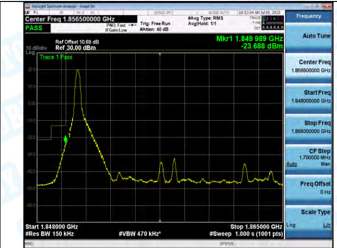
Band2_Band2_15MHz_16QAM_18675_1RB#0
