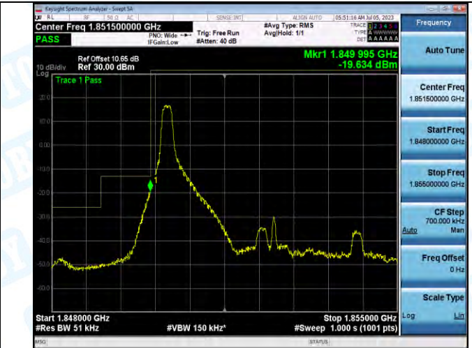
Band2_Band2_5MHz_16QAM_18625_1RB#0
