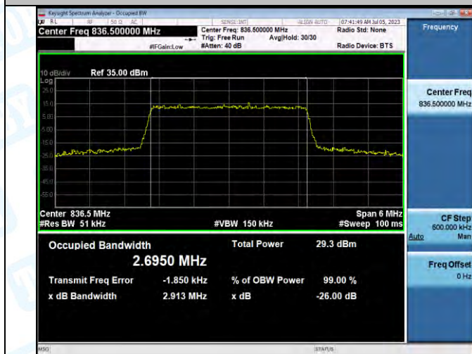
Band5-3MHz-QPSK-20525-15RB#0-PASS
