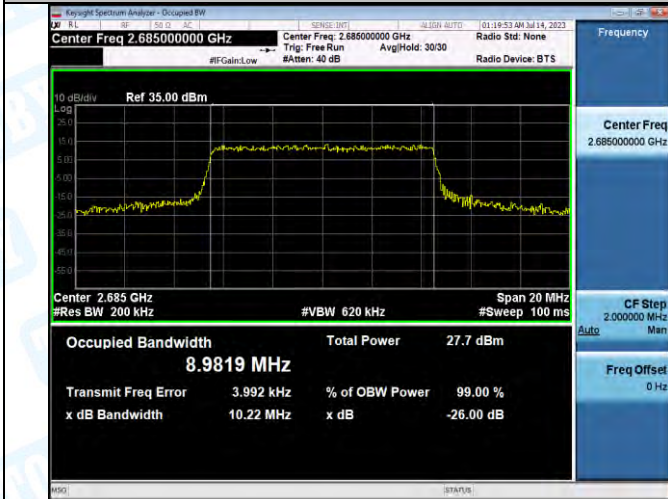
Band41-10MHz-QPSK-41540-50RB#0-PASS
