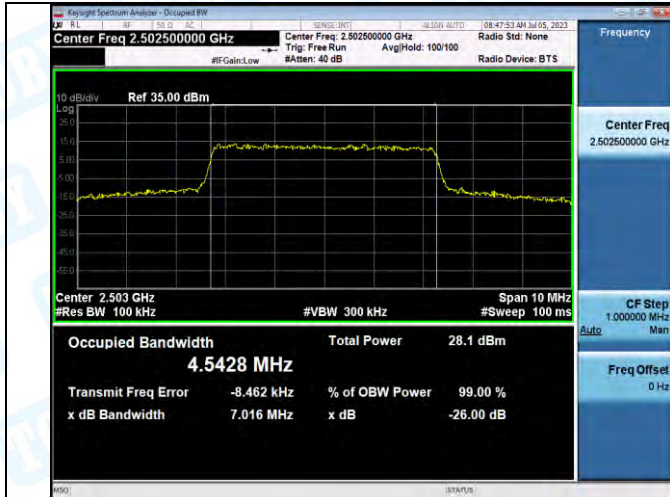
Band7-5MHz-QPSK-20775-25RB#0-PASS
