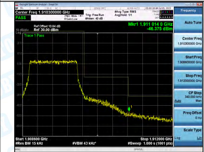
Band2_Band2_1.4MHz_16QAM_19193_6RB#0
