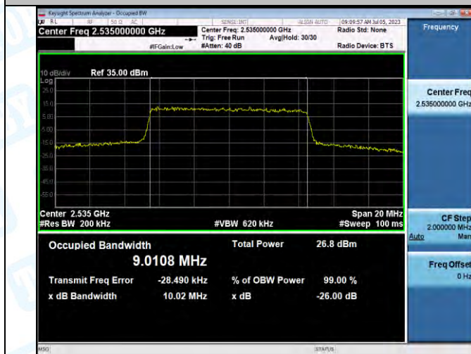
Band7-10MHz-QPSK-21100-50RB#0-PASS
