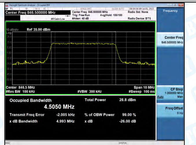
Band5-5MHz-16QAM-20625-25RB#0-PASS
