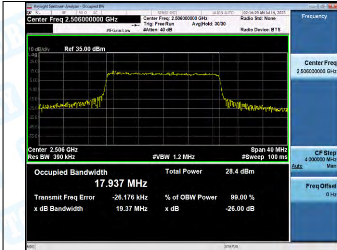
Band41-20MHz-QPSK-39750-100RB#0-PASS
