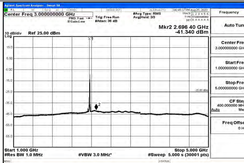
Band7-15MHz-16QAM-21375-1RB#0-Range5:5000~12000MHz
