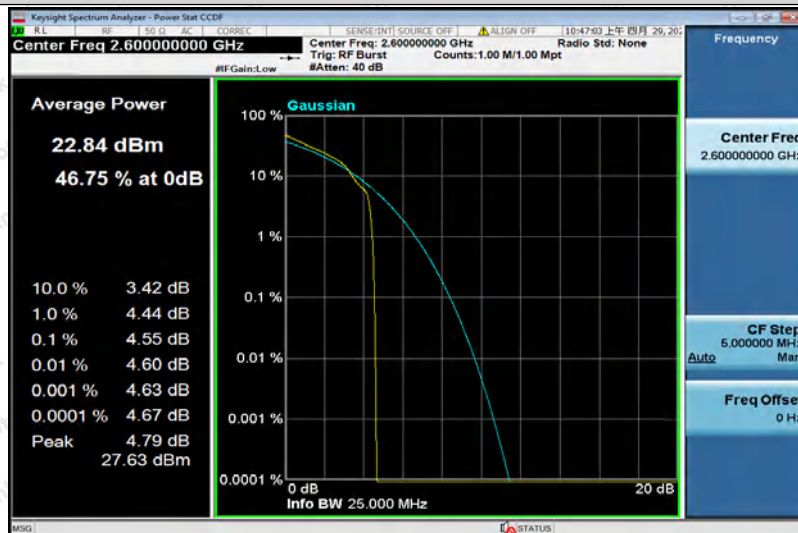
Band41-20MHz-16QAM-40690-100RB#0
