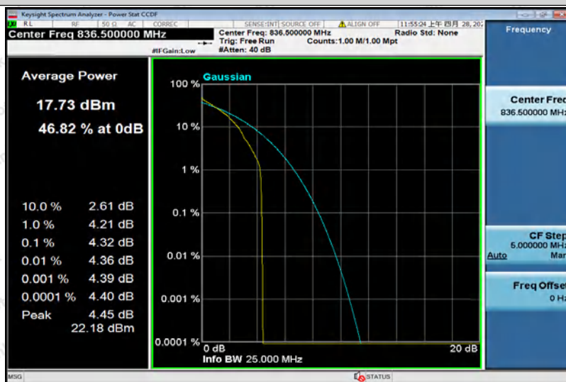
Band5-5MHz-QPSK-20525-25RB#0
