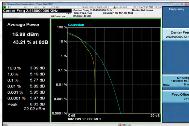
Band7-15MHz-16QAM-21100-75RB#0
