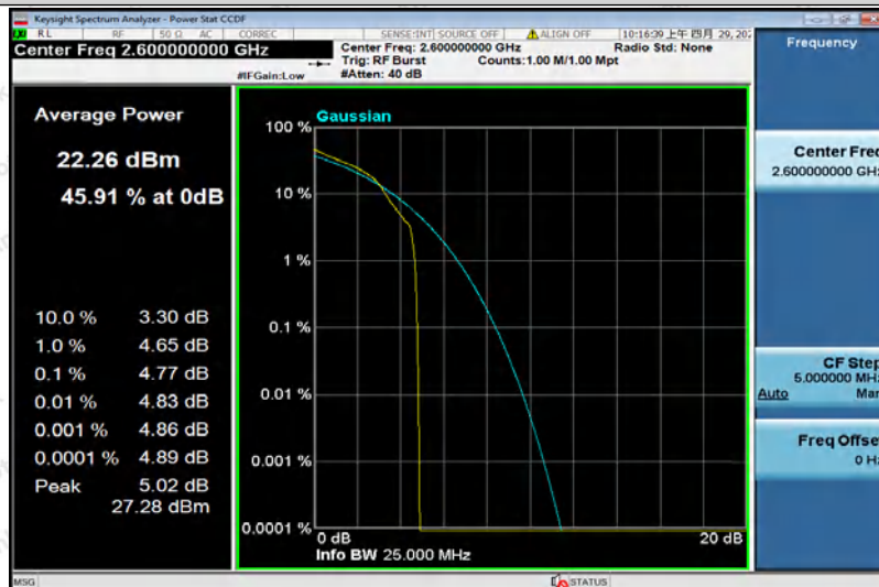
Band41-15MHz-16QAM-40690-75RB#0
