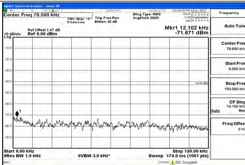
Band2-3MHz-16QAM-18900-1RB#0-Range2:0.15~30MHz
