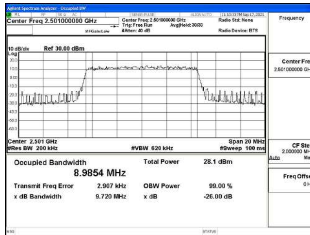
Band41-10MHz-16QAM-40620-50RB#0
