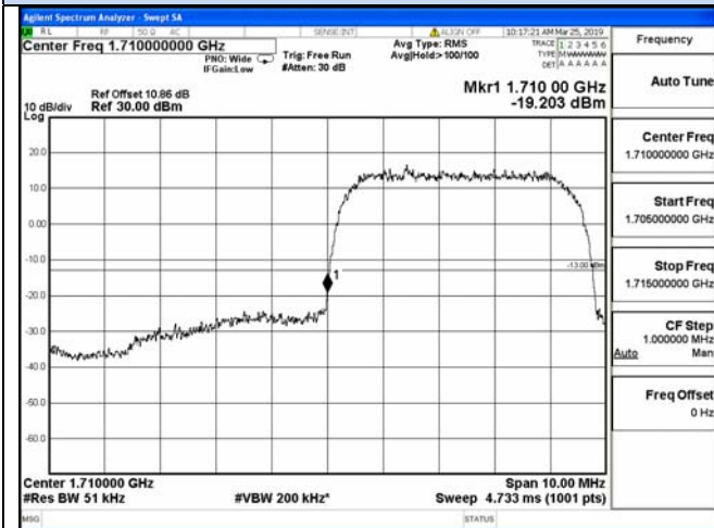
Channel 1312 / 1713 MHz
