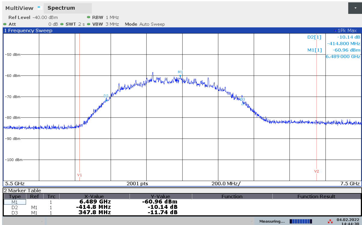
Plot 17: +10 °C, Vnom
