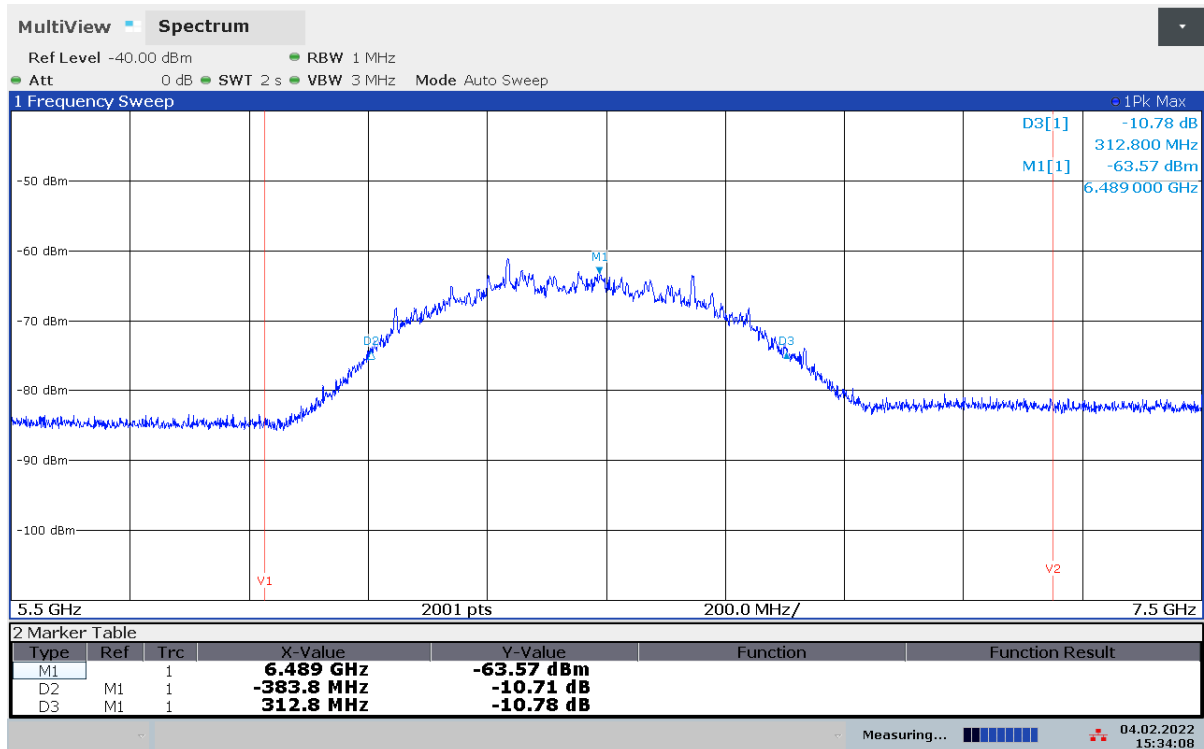
Plot 23: +50 °C, Vnom
