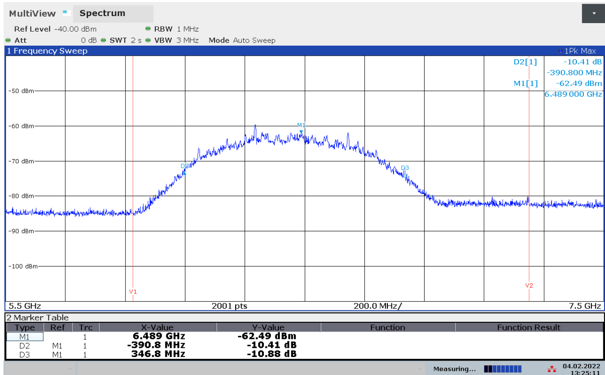
Plot 19: +20 °C, Vnom
