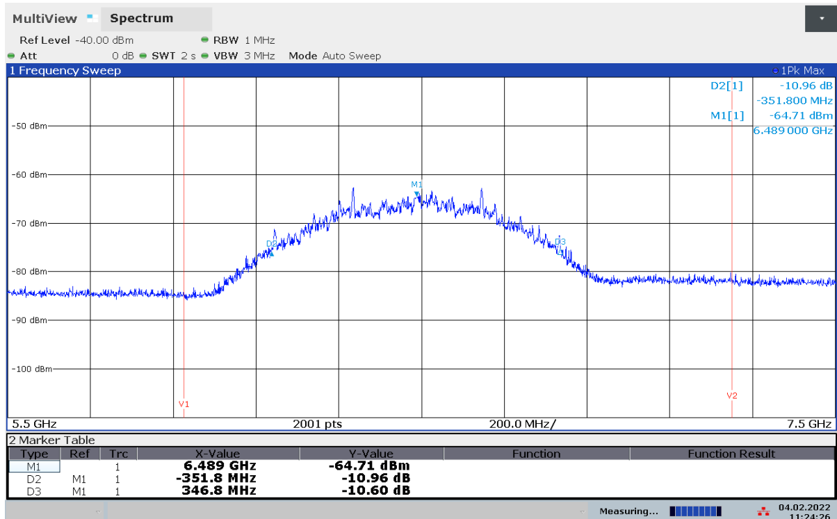
Plot 20: +20 °C, Vmax
