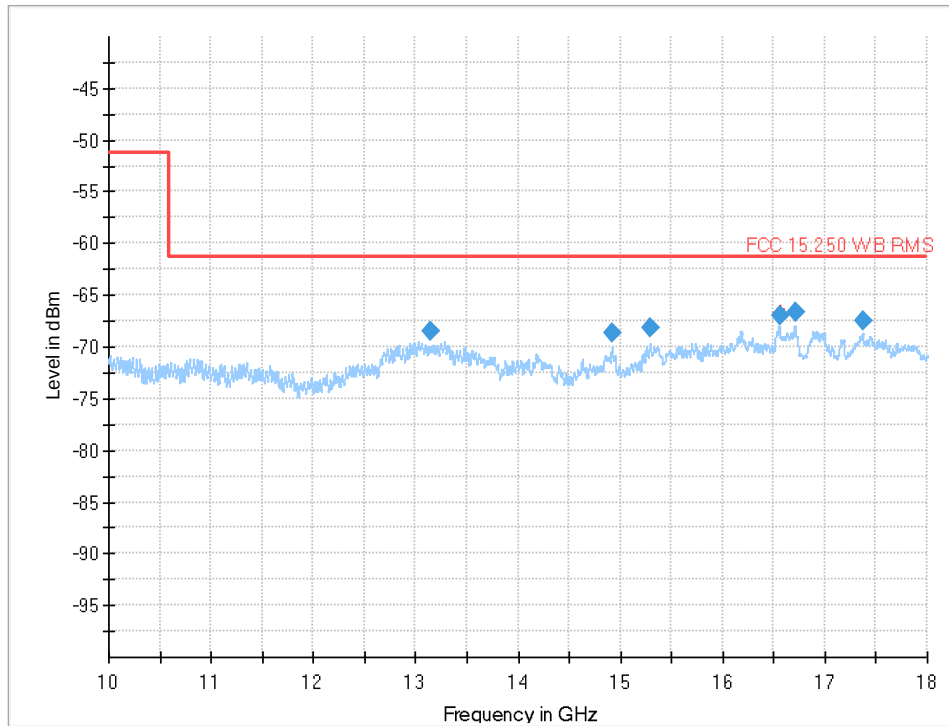
Plot 8: 10 GHz to 18 GHz
