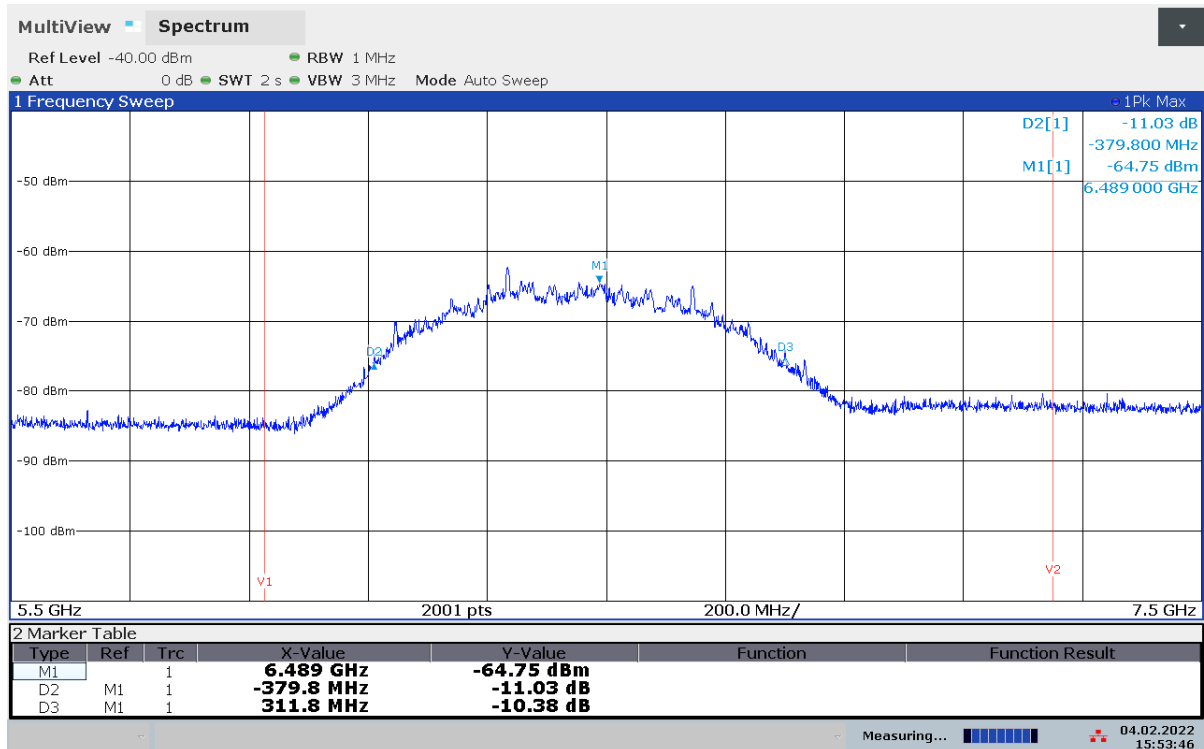
Plot 24: +60 °C, Vnom
