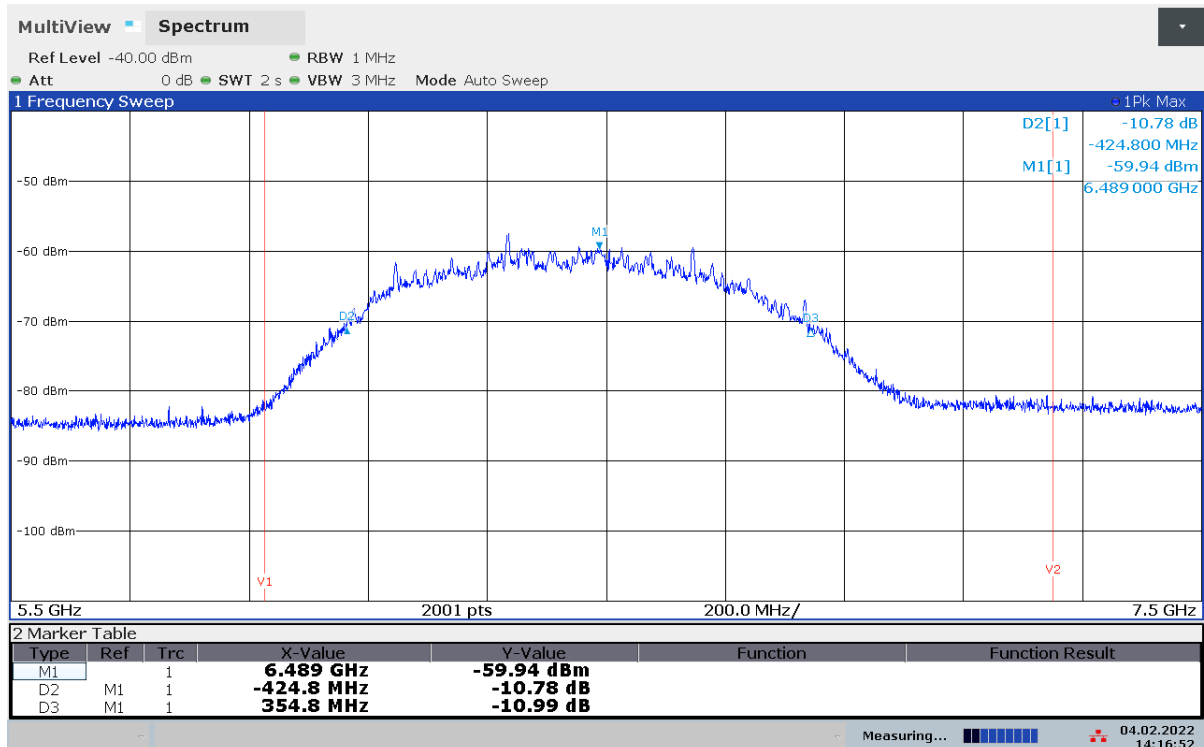
Plot 16: 0 °C, Vnom
