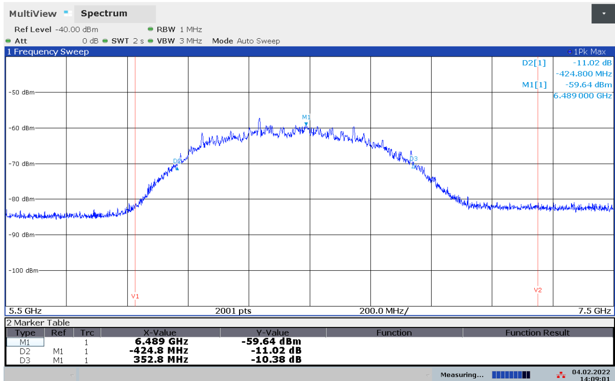
Plot 15: -10 °C, Vnom
