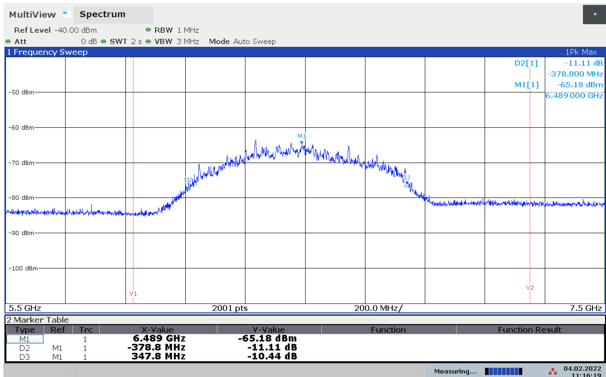
Plot 18: +20 °C, Vmin = 3.25 V (Note: below this value the DUT switches off automatically)
