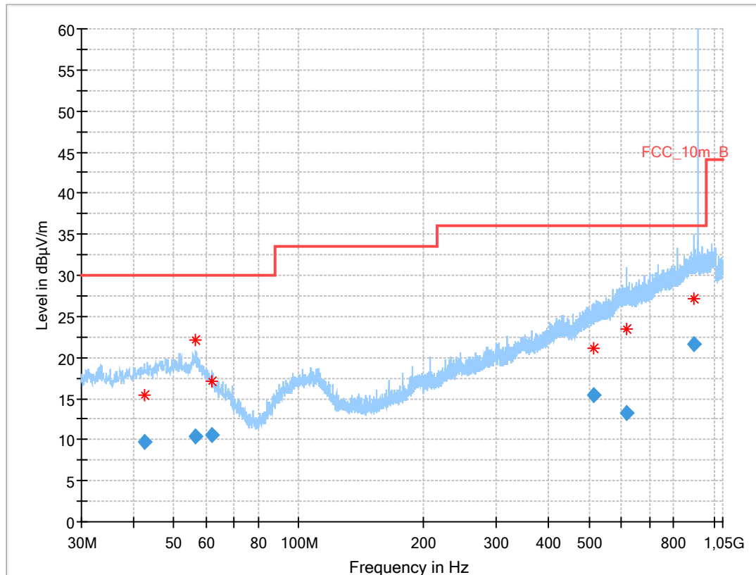
Plot 1: 30 MHz to 1 GHz, vertical & horizontal polarization
