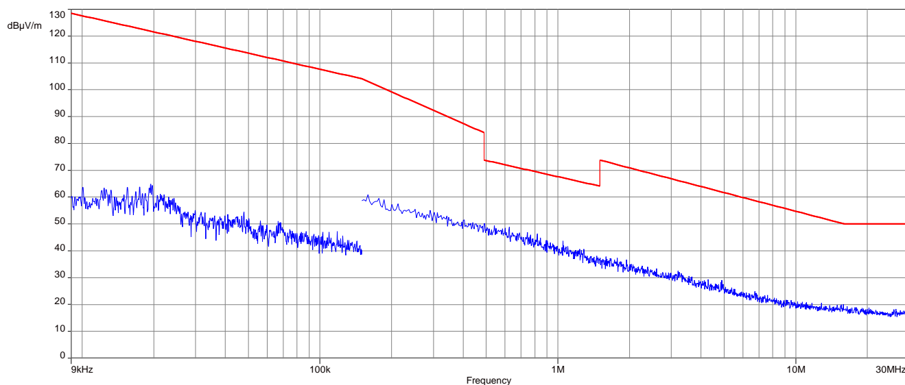
Plot 1: 9 kHz to 30 MHz
