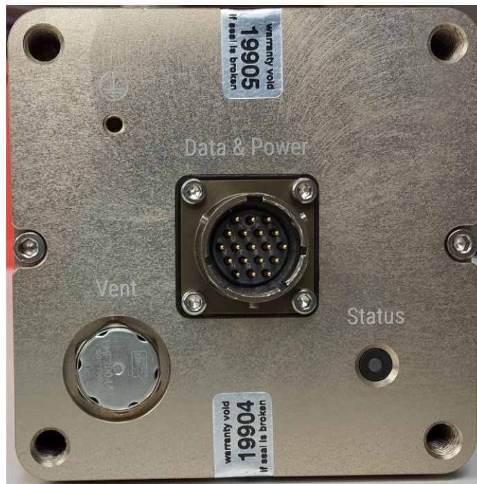
Figure 5: iLDR-M-G5-DN100
