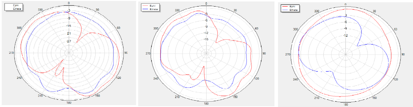
Antenna pattern for 2440MHz
