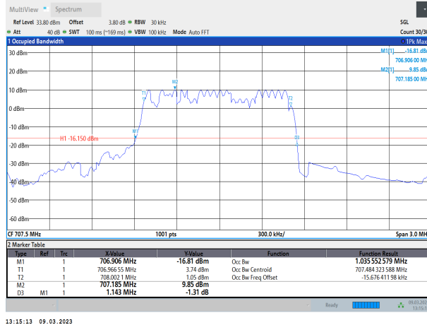
Band12-1.4MHz-QPSK-23095-6RB#0
