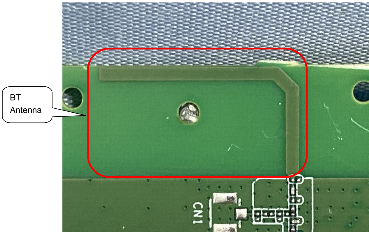
INTERNAL VIEW OF EUT (FIGURE 13)
