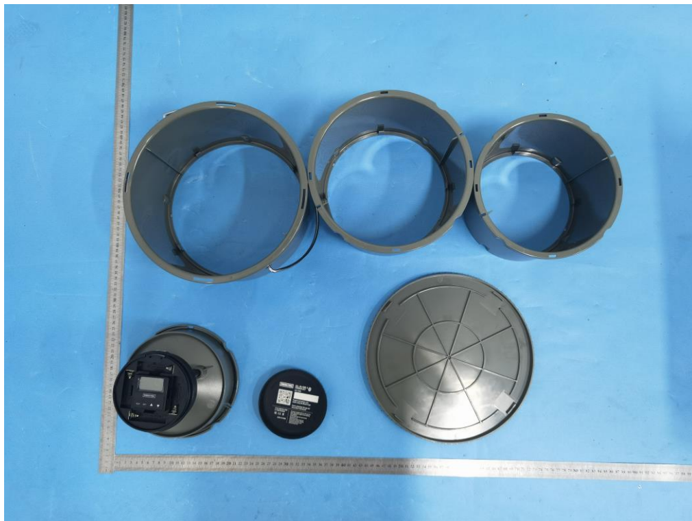
Series Model: MFG-15100 OPEN VIEW OF EUT(FIGURE 1)
