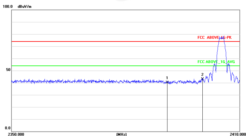
2402MHz Vertical
