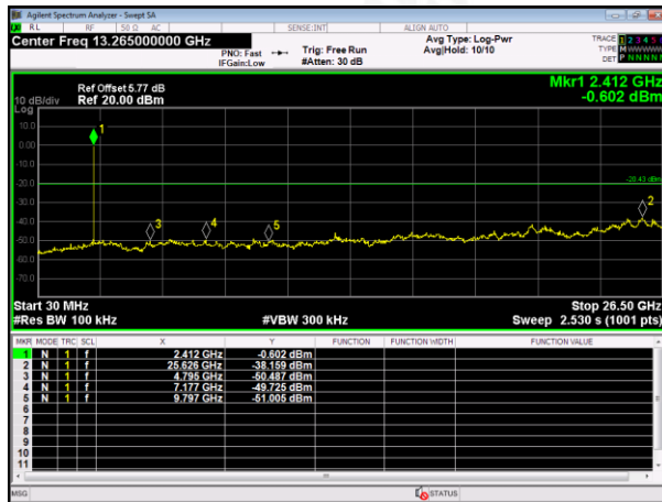
802.11b-Lowest channel
