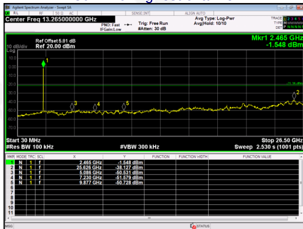
802.11b-Highest channel
