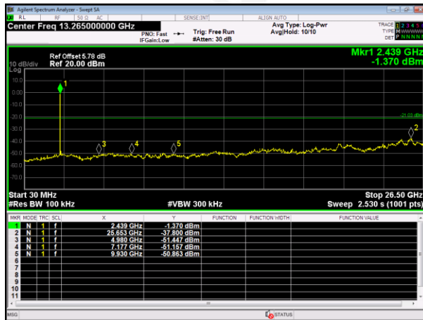
802.11b-Middle channel
