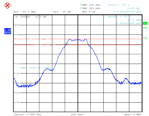
BLE_1M_Low_Channel
