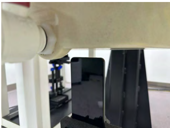
Bottom Side of EUT with 1.7 cm Gap (Extremity Mode)
