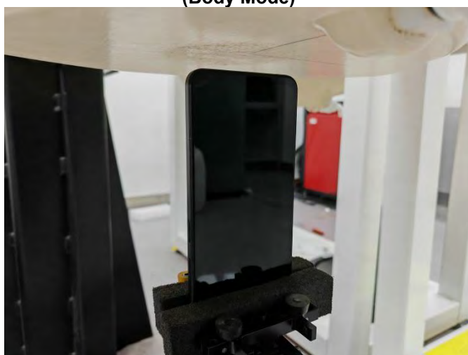
Bottom Side of EUT with 1 cm Gap (Body Mode)
