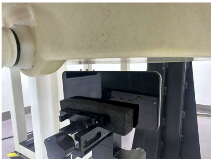
Left Side of EUT with 1.3 cm Gap (Extremity Mode)
