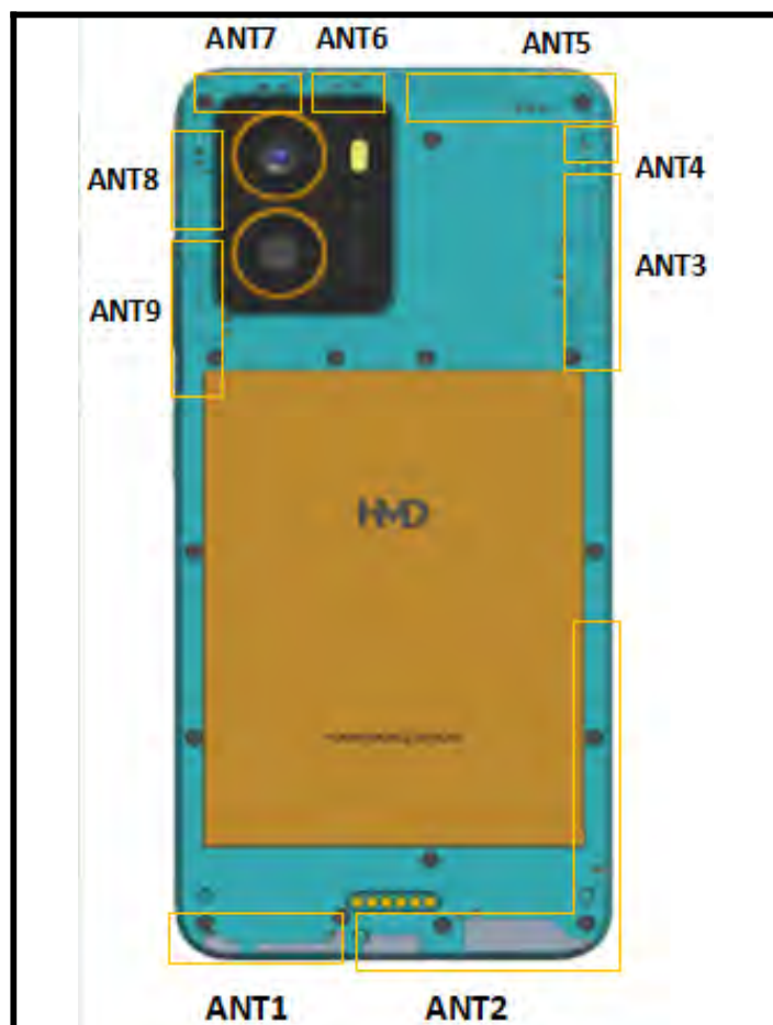
<EUT Rear View>
