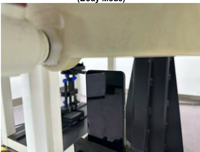
Top Side of EUT with 2.2 cm Gap (Extremity Mode)
