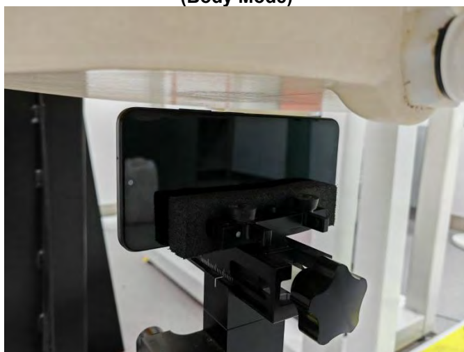
Right Side of EUT with 1 cm Gap (Body Mode)
