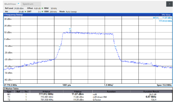
Band13-5MHz-256QAM-23255-25RB#0
