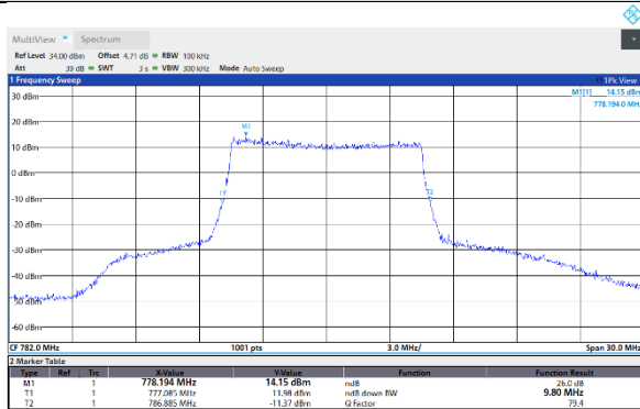
Band13-10MHz-16QAM-23230-50RB#0
