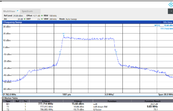
Band13-10MHz-16QAM-23230-50RB#0
