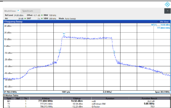
Band13-10MHz-256QAM-23230-50RB#0
