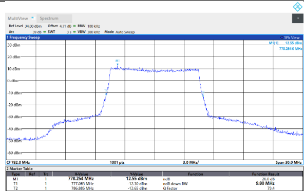
Band13-10MHz-256QAM-23230-50RB#0
