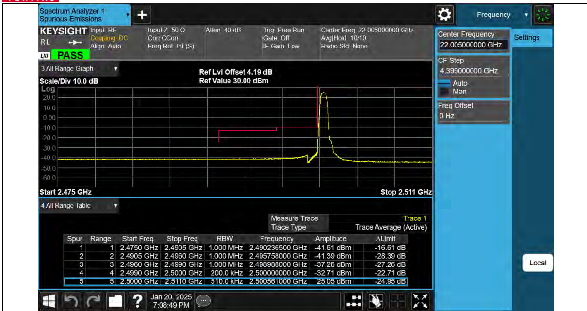
Band7-10MHz-QPSK-20800-50RB#0-PASS
