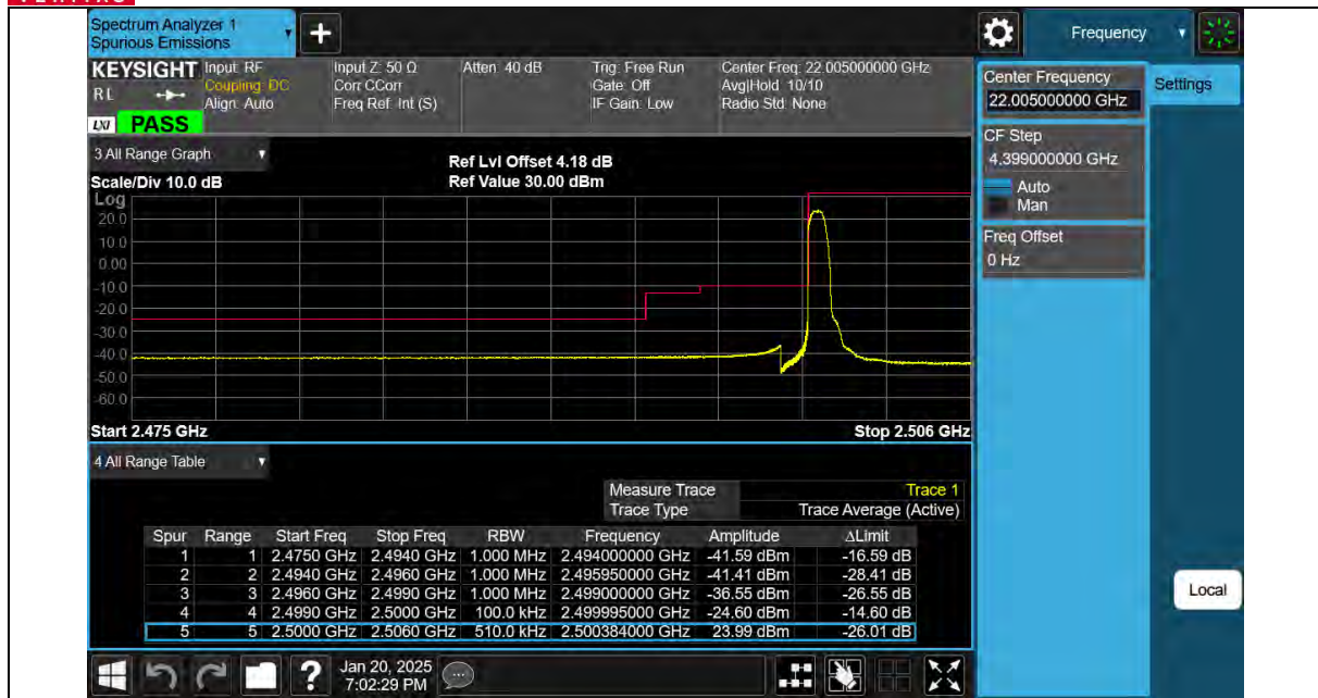
Band7-5MHz-16QAM-20775-25RB#0-PASS
