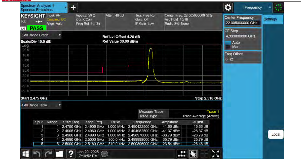
Band7-15MHz-16QAM-20825-75RB#0-PASS
