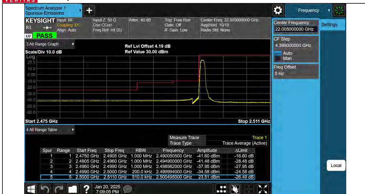
Band7-10MHz-16QAM-20800-50RB#0-PASS
