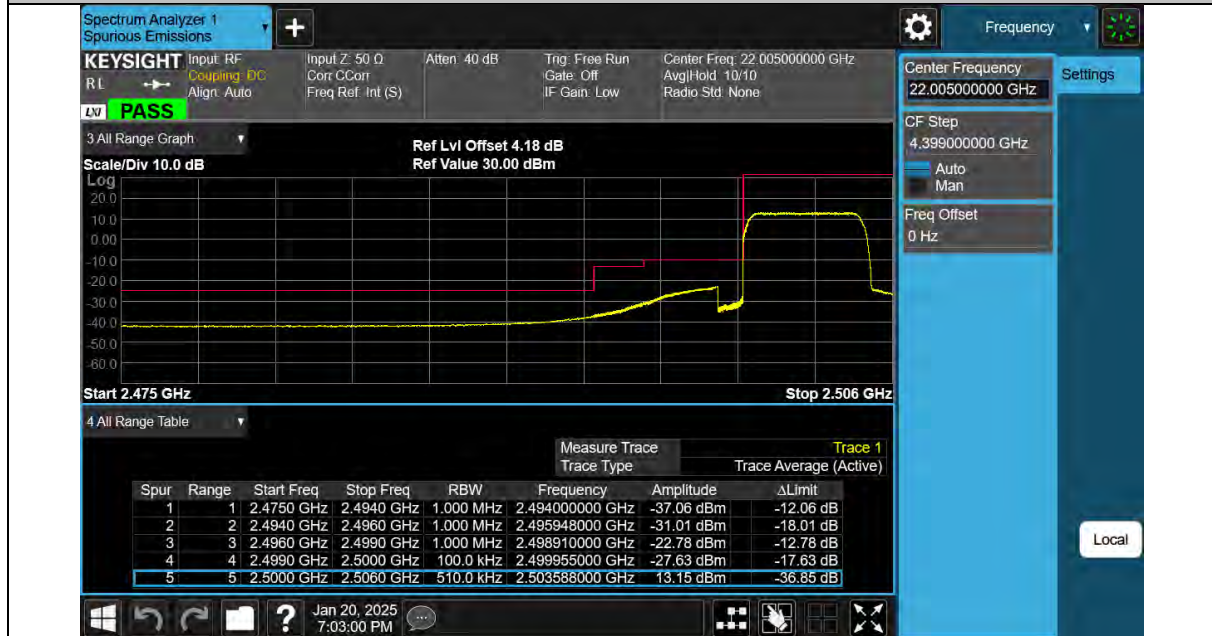
Band7-5MHz-16QAM-21425-25RB#0-PASS
