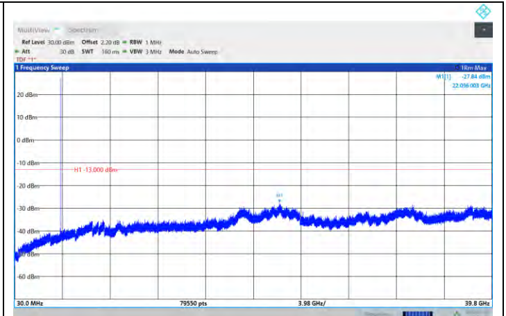
N77-3700-3980-PC2-30-20-M-DFT-QPSK-Edge 1RB Left
