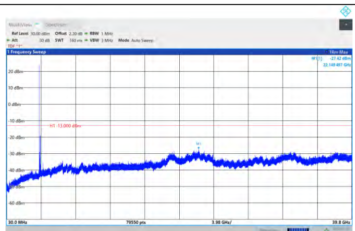
N77-3700-3980-PC2-30-100-M-DFT-QPSK-Edge_1RB_Left
