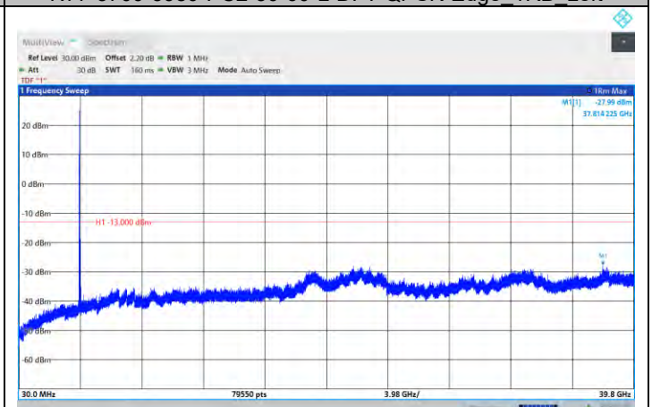
N77-3700-3980-PC2-30-60-H-DFT-QPSK-Edge 1RB Left
