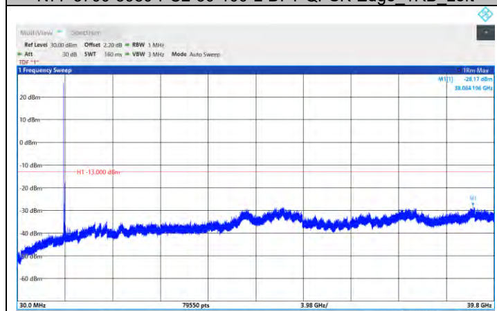
N77-3700-3980-PC2-30-100-H-DFT-QPSK-Edge_1RB_Left
