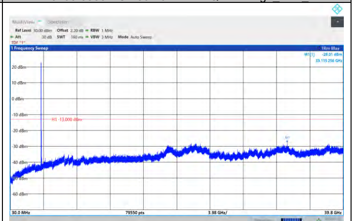
N77-3700-3980-PC2-30-60-L-DFT-QPSK-Edge 1RB Left
