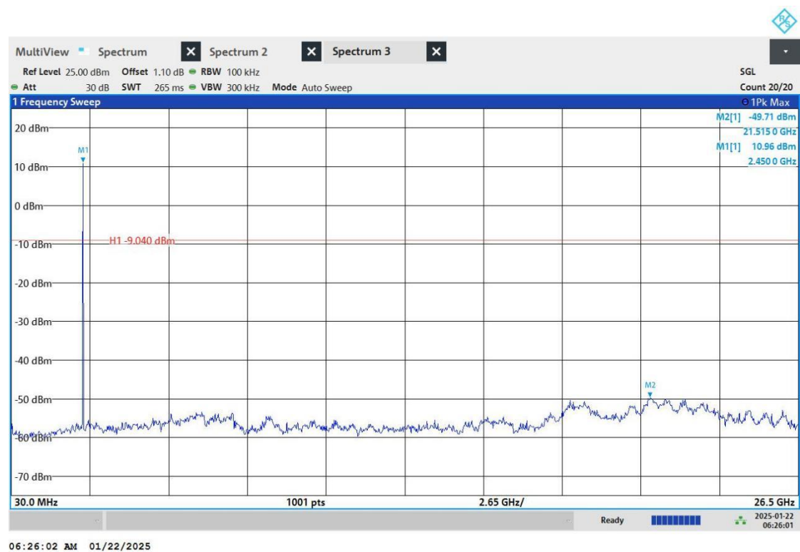
DH5_ANT7_2441_30~26500
