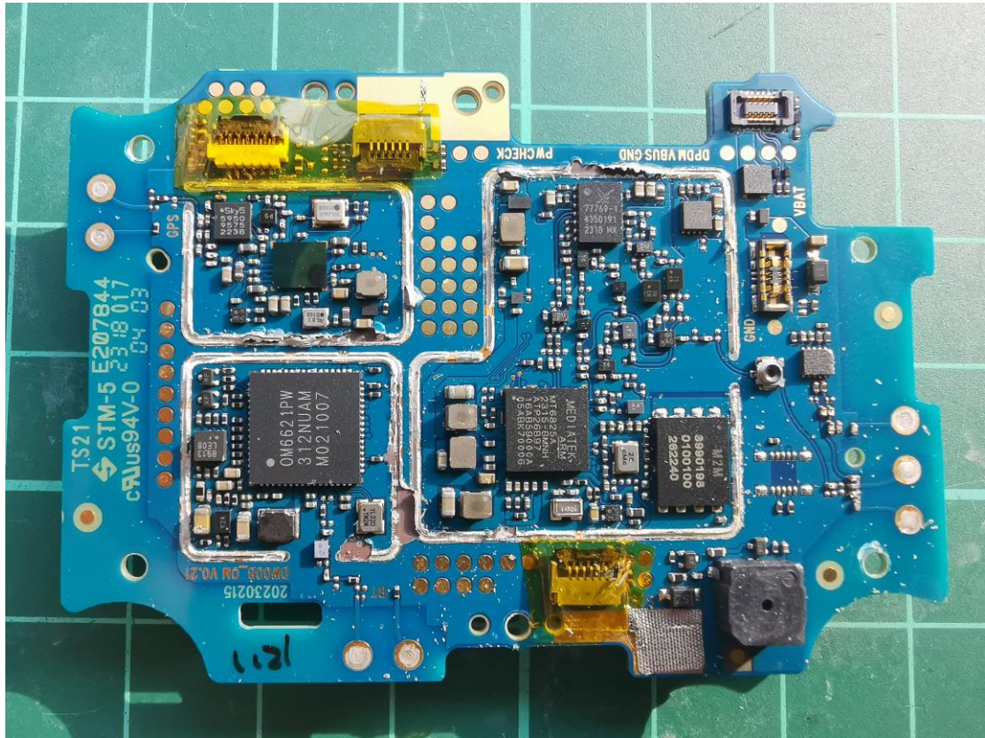
TA-1698 Mobile Phone Disassembly
