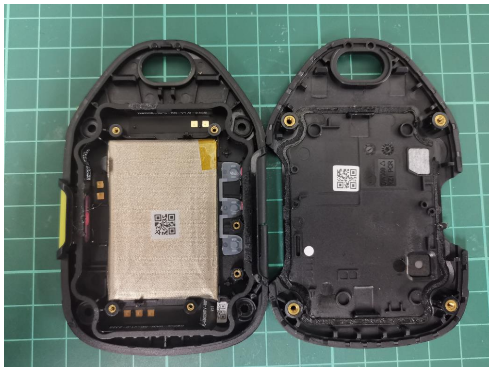
TA-1698 Mobile Phone Disassembly
