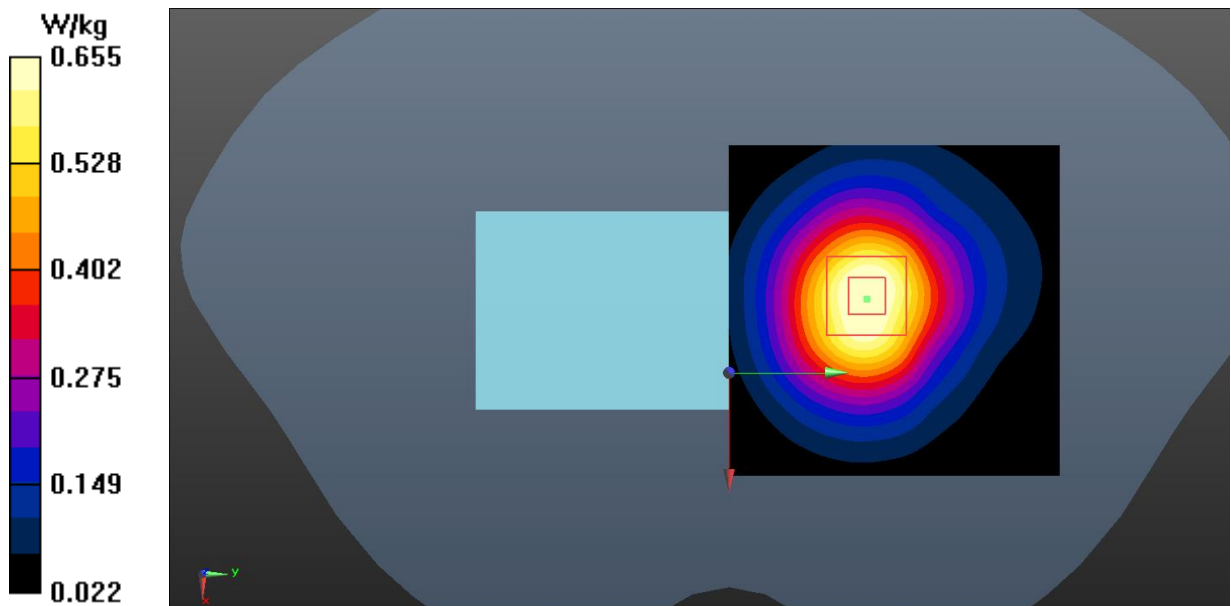
Fig.4 GSM 1900 Body
