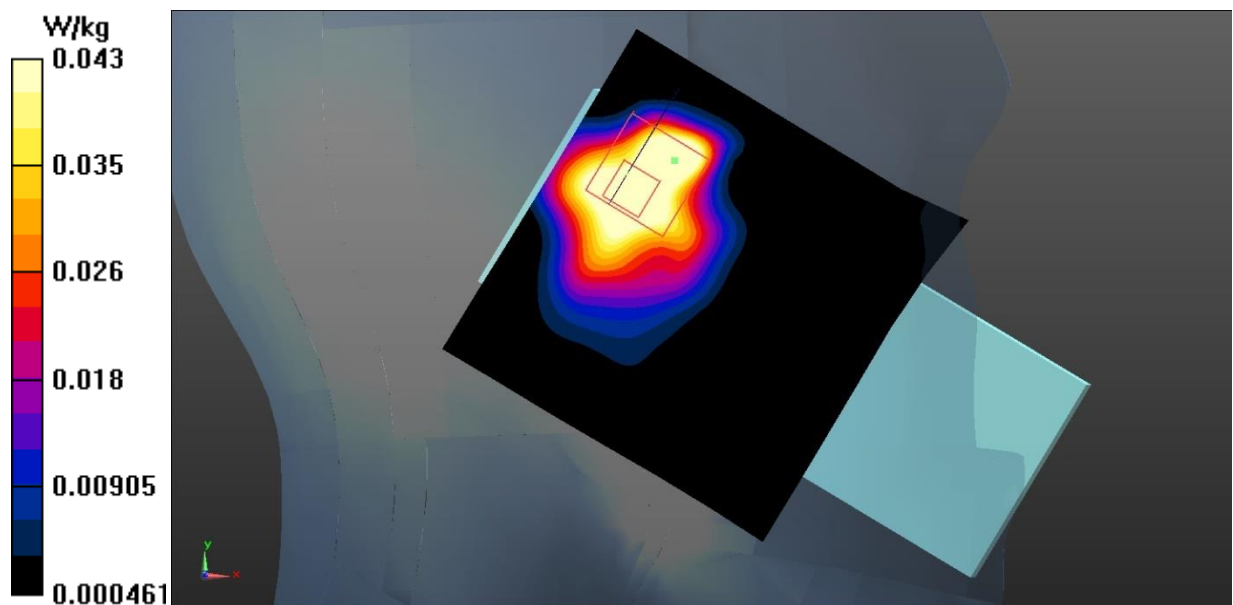
Fig.19 Bluetooth Head
