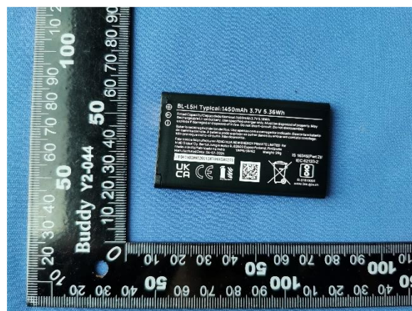
Fenghua- HMD logo Battery2-1
