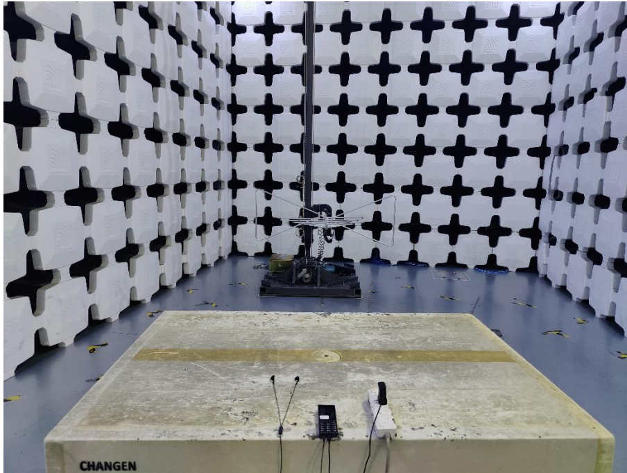
1. Radiated Emissions (Part 15B Video Player,30MHz-1GHz)
