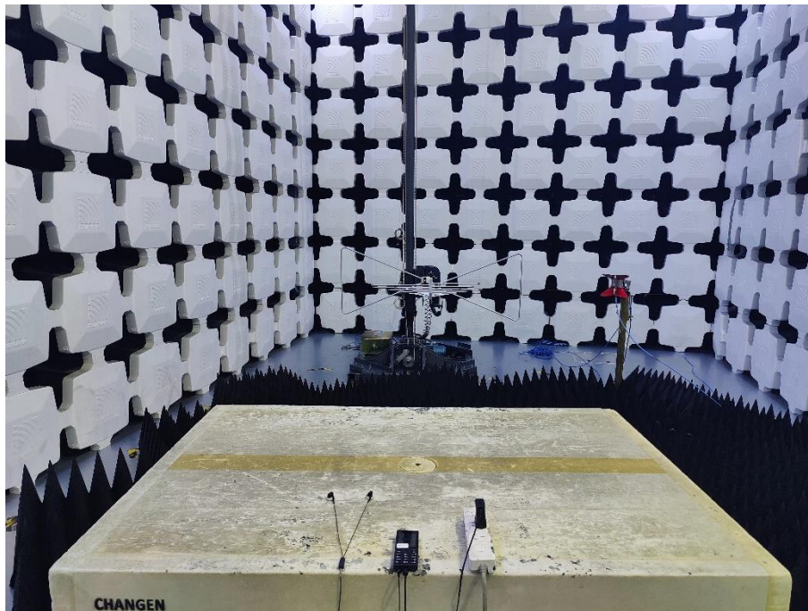
2. Radiated Emissions (Part 15B Video Player,1GHz-18GHz)
