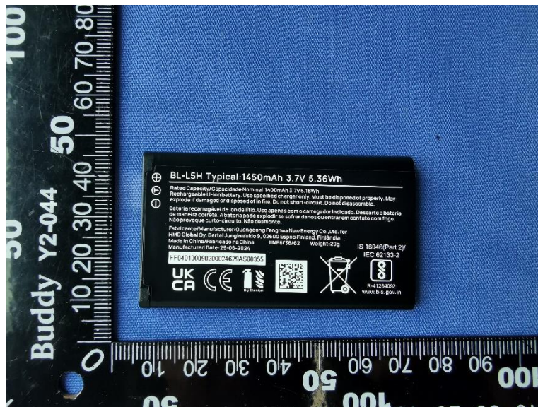
Fenghua- HMD logo Battery2-3
