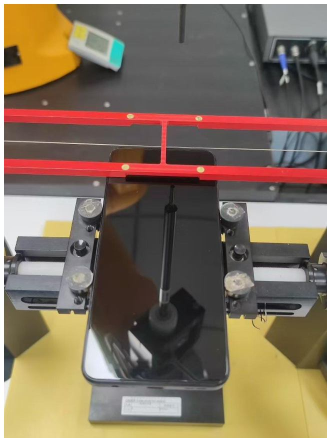
Picture 2: EUT Positioning for T-coil
