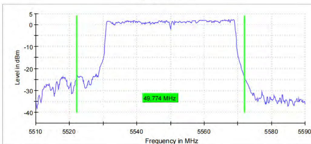
26 dB Bandwidth
