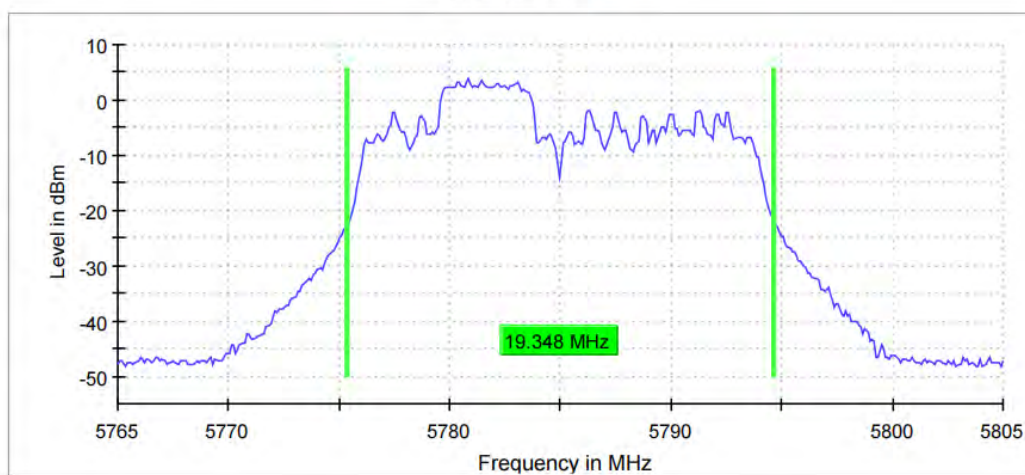
26 dB Bandwidth
