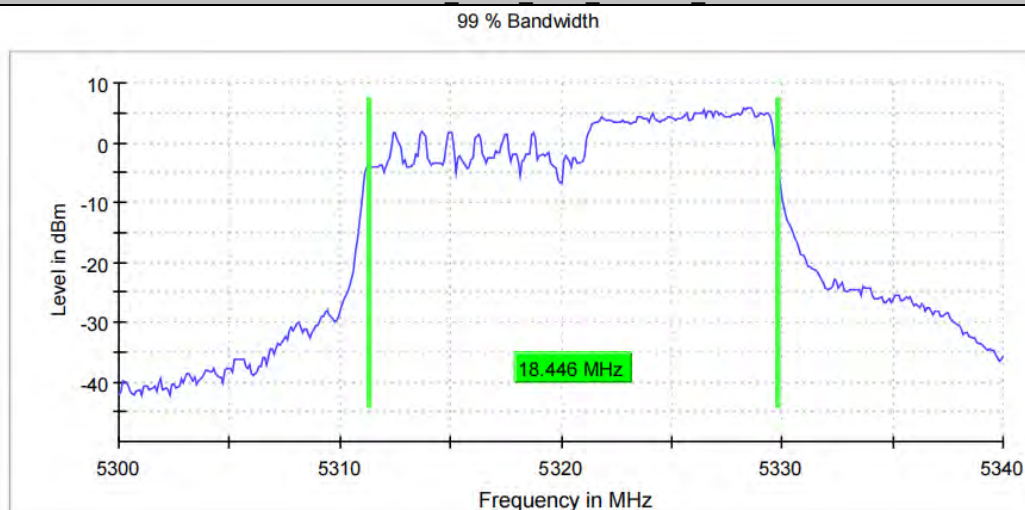
11AX20MIMO Ant11 5320 106Tone RU54
