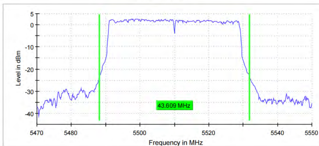
26 dB Bandwidth
