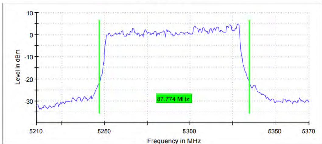
26 dB Bandwidth
