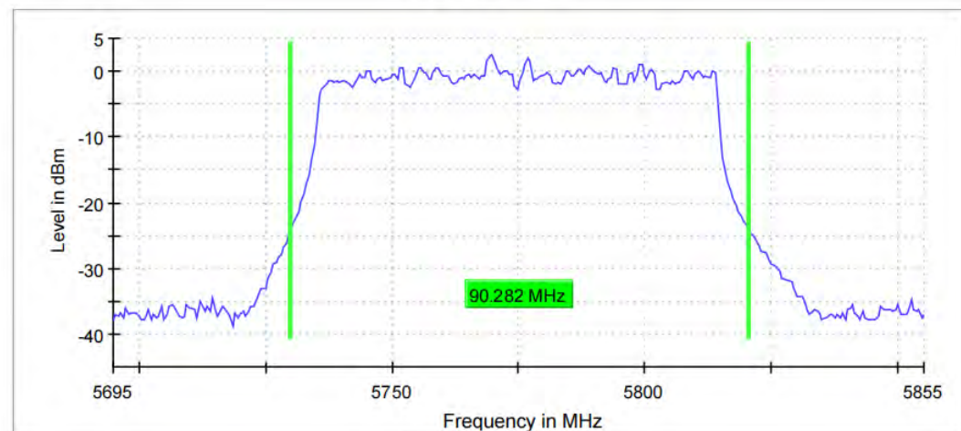
26 dB Bandwidth
