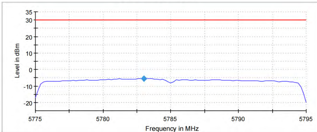
11AX20 Ant11 5785 Power Spectral Density (SA-1)
