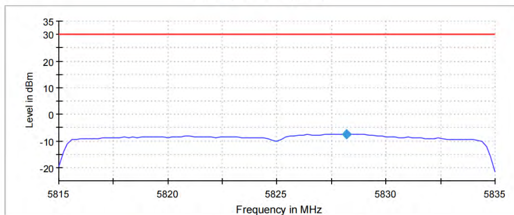
11AX20 Ant8 5825 Power Spectral Density (SA-1)
