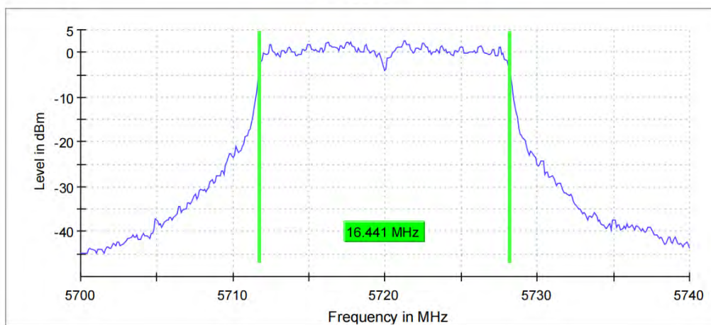
99 % Bandwidth
