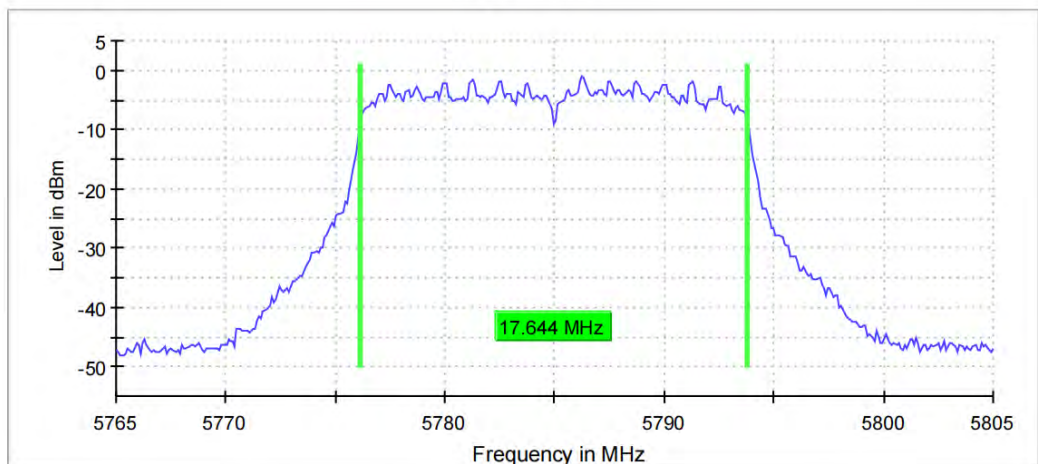
99 % Bandwidth
