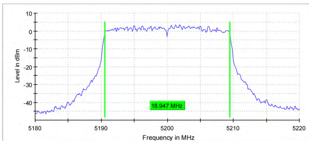
99 % Bandwidth
