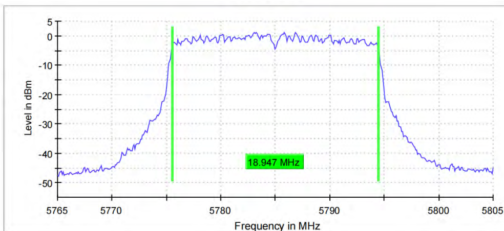
99 % Bandwidth
