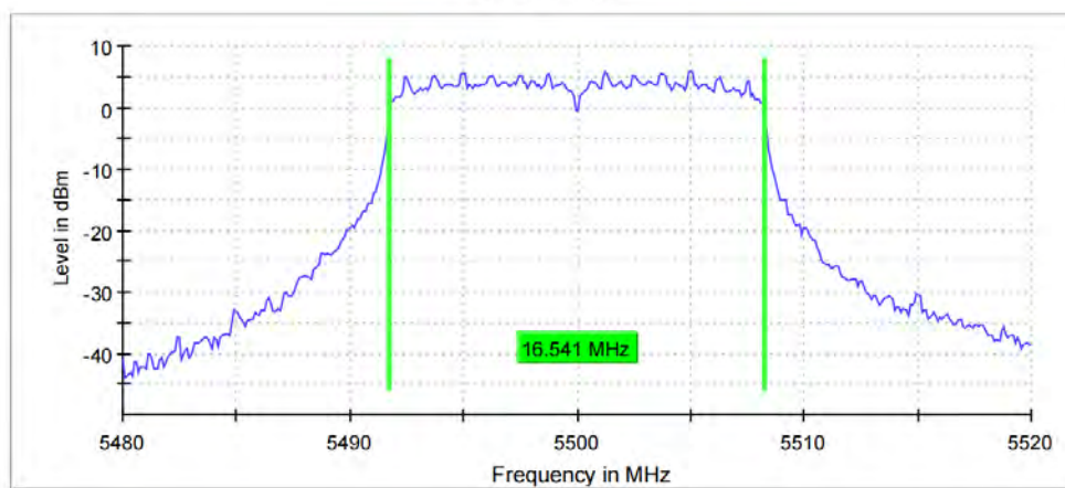
99 % Bandwidth
