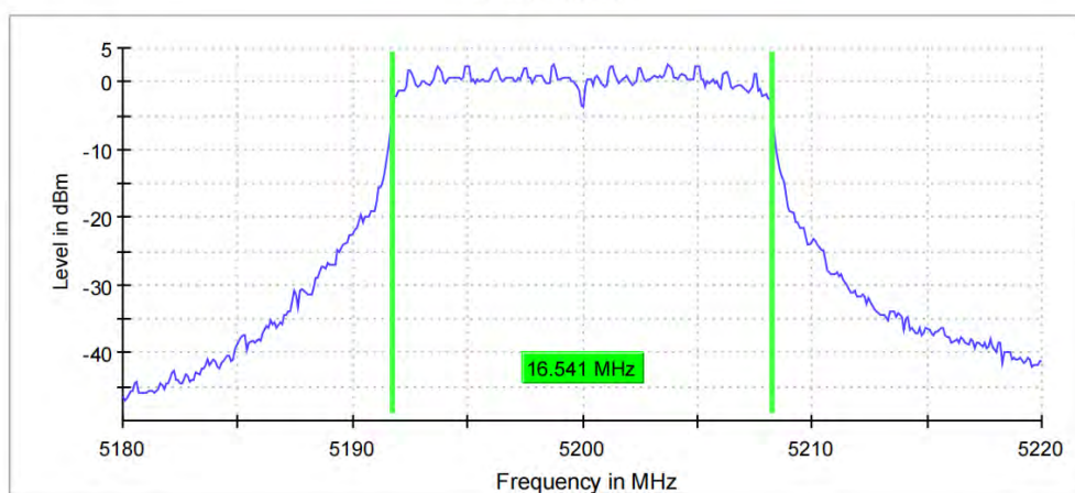
99 % Bandwidth
