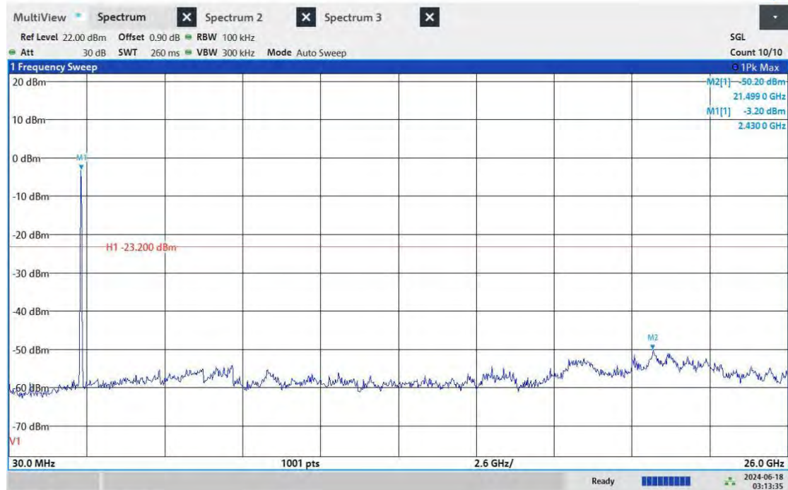
11AX40_Ant9_2452_30~26000
