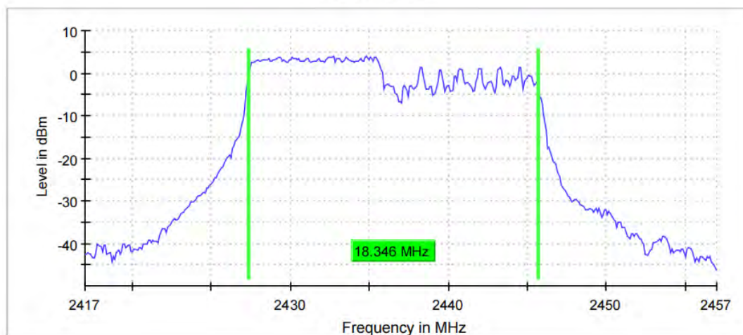
99 % Bandwidth
