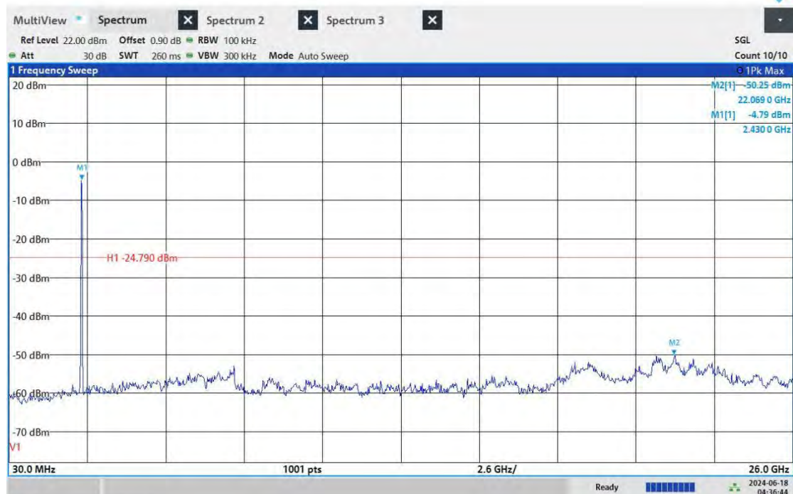
11AX40_Ant10_2437_30~26000
