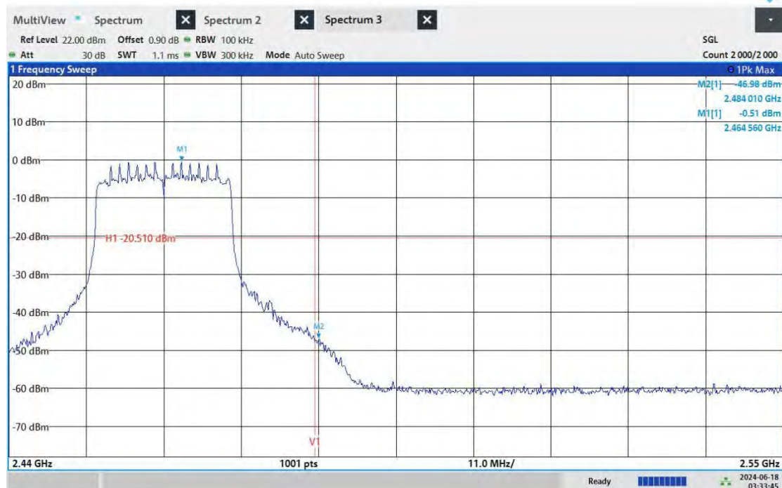
11AX20_Ant10_High_2462
