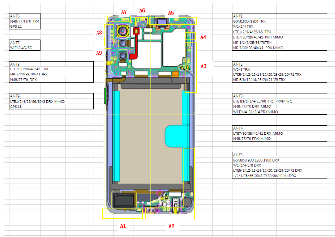
Picture 15: Antenna Locations
