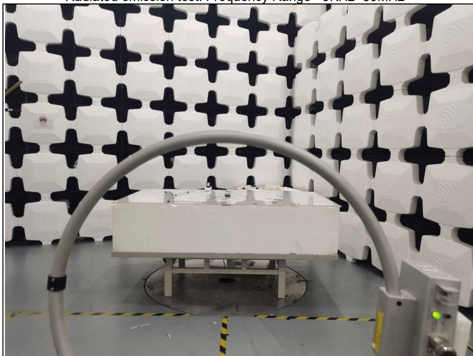
Radiated emission test: Frequency Range < 9KHz- 30MHz >
