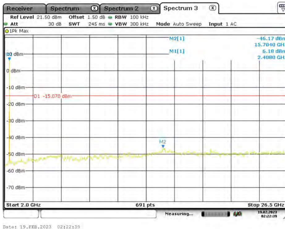
3DH5_Ant1_2402_2000~26500
