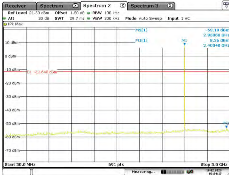
3DH5_Ant1_2402_30~3000
