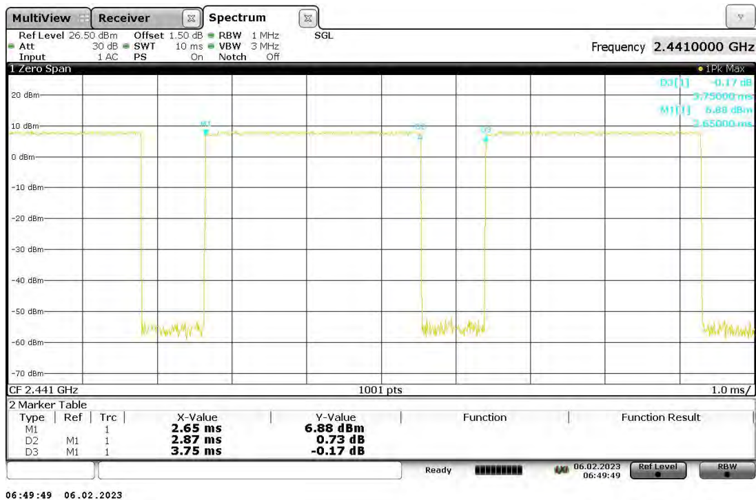
2DH5_Ant1_2441
