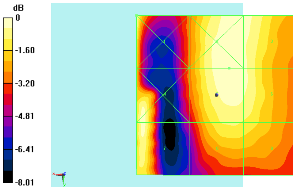
Fig B.4 HAC RF E-Field LTEB41 PC3
