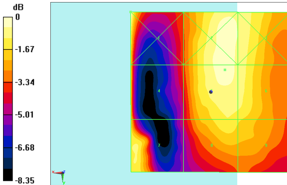
Fig B.3 HAC RF E-Field LTEB41 PC2
