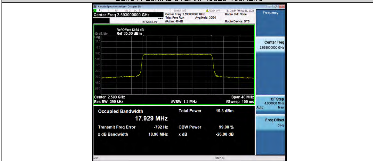
Band41-20MHz-64QAM-41490-100RB#0
